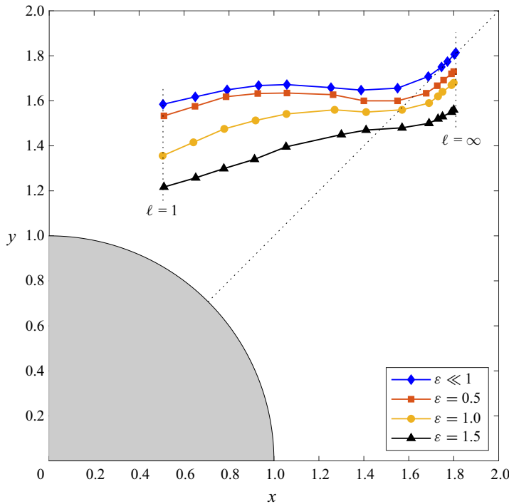
Figure 7. The variation with the inter-cylinder distance \ell of the location of the Lagrangian vortex centre x_c for M=2 as determined in the limit \varepsilon \ll 1 and as determined from the DNS computations with \varepsilon = (0.5, 1.0, 1.5) . The symbols represent the results corresponding to \ell = (1, 1.25, 1.5, 1.75, 2, 2.5, 3, 4, 6, 8, 10, 15, \infty) .
