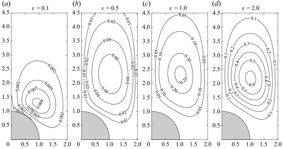
Figure 11. The relative error |(\psi_{SS} - \langle \psi \rangle / \epsilon) / \psi_{SS, peak}| corresponding to \ell = 2 and M = 2 for different values of the stroke length \epsilon .
