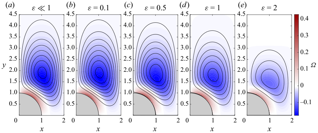
Figure 3. Streamlines and colour contours of vorticity \Omega for \ell = 2 and M = 2 . Besides results corresponding to the steady-streaming velocity \mathbf{v}_{SS} , shown in panel (a), results are given for the rescaled time-averaged Eulerian velocity \langle \mathbf{v} \rangle / \varepsilon determined in the DNS computations for \varepsilon = (0.1, 0.5, 1.0, 2.0) in panels (b)–(e). Streamlines are represented using a constant spacing \delta\psi = 0.005 . Corresponding vorticity levels are indicated in the colour bar on the right.
