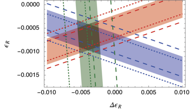
Fig. 2. Constraints in the \Delta\epsilon_R - \epsilon_R plane from the \Delta_{\text{CKM}}^{(i)} introduced in Eq. (8). The bands with positive slope (red) correspond to \Delta_{\text{CKM}}^{(1)} . The bands with small negative slope (blue) correspond to \Delta_{\text{CKM}}^{(2)} , while the bands with steep negative slope (green) correspond to \Delta_{\text{CKM}}^{(3)} . The filled bands reflect the current situation (11), the long-dashed ones the +2\sigma scenario (12), and the short-dashed ones the opposite case (13). Note that in each case the three bands essentially overlap by construction, since V_{ud} , V_{us} , subject to the unitarity constraint, and the BSM contamination via \Delta\epsilon_R , \epsilon_R , amount to three free parameters. The main impact of the proposed new measurement of the K_{\mu 3}/K_{\mu 2} branching fraction thus concerns a corresponding shift in the \Delta_{\text{CKM}}^{(3)} band if the \pm 2\sigma scenarios were realized.
