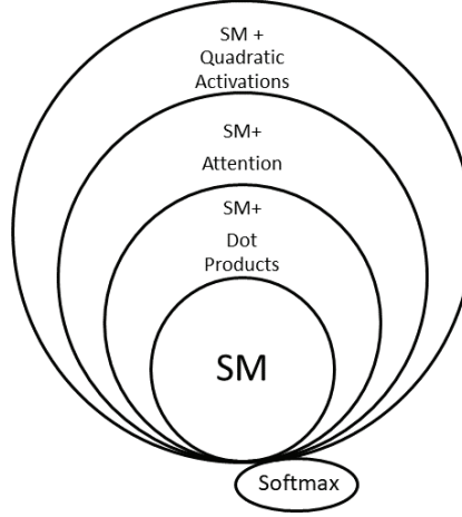
Figure 18. Standard model and some of its extensions.
