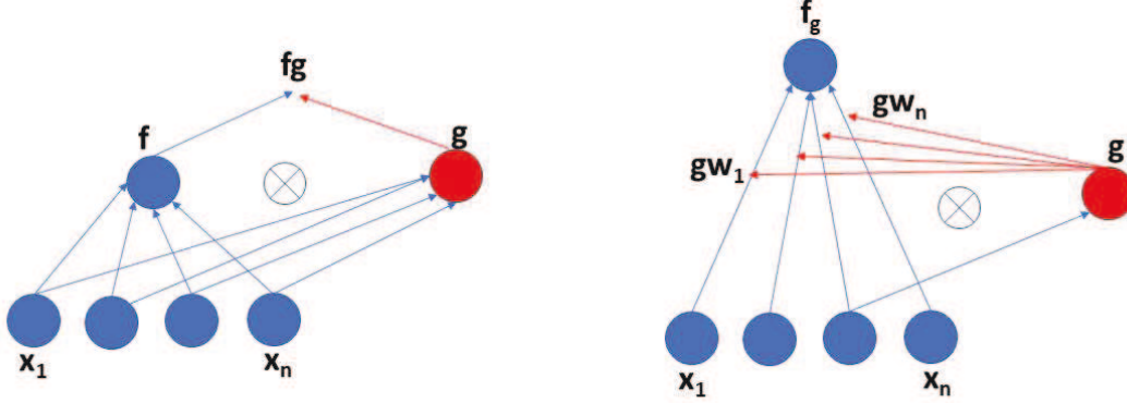
Figure 13. Left: Output gating with a single attention unit. Both the gated function f and the gating function g are linear (or polynomial) threshold gates of the same input vector x = (x_1, \dots, x_n) . The overall network computes the function f_g(x) = f(x)g(x) . Right: Synaptic gating with a single attention unit g(x) gating all the incoming weights of the gated function f(x) . So the overall network computes the function f_g(x) . For instance, if f is a linear threshold gate f(x) = \text{sign}(\sum_i w_i x_i) , then f_g(x) = \text{sign}(\sum_i g(x) w_i x_i) .
