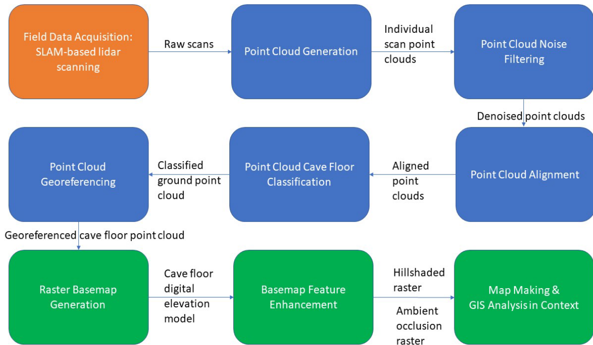
Figure 5. Overview of processing workflow.
