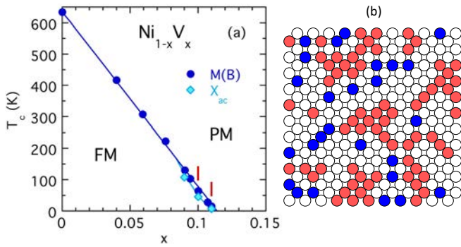
FIG. 1. (a) Magnetic phase diagram of \text{Ni}_{1-x}\text{V}_x displaying the critical temperature T_c vs vanadium concentration x separating the ferromagnetic ordered phase (FM) from the paramagnetic phase (PM) leading to a quantum critical point [26]. The red markers indicate the samples for this investigation. The right panel (b) demonstrates the magnetic inhomogeneities in \text{Ni}_{1-x}\text{V}_x with x = 0.10 in an fcc lattice plane: it shows how randomly placed V atoms (in blue) separate Ni-rich regions (in red) responsible for magnetism. Since V affects more the moment of the local Ni neighbors, we distinguish these close Ni sites (in white) from the rest, the more distant Ni atoms (in red).
