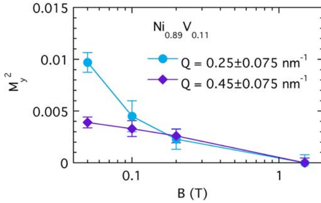
FIG. 9. Field dependence of magnetic component M_y^2 of \text{Ni}_{0.89}\text{V}_{0.11} at low T = 4 K. M_y^2 values estimated from \text{SF}(\theta) using Eq. (1) at two different Q ranges as indicated. Lines just connect data.
