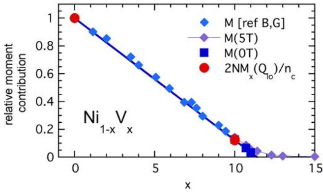
FIG. 17. Relative moment contribution vs vanadium concentration x from SANS results and other methods from Ref. [26]. 2NM_x(Q_{\text{low}})/n_c and bulk magnetization data M(B) normalized to the value of Ni are shown. The long-range ordered domain term follows the trend of the linear reduction of the average magnetic moment with x .
