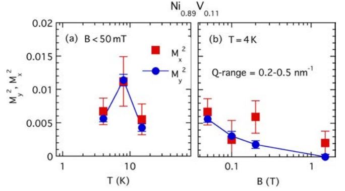
FIG. 8. Magnetic components M_y^2 and M_x^2 extracted from fit [Eq. (1)] of \text{SF}(\theta) data (shown in Fig. 6) of \text{Ni}_{0.89}\text{V}_{0.11} with T_c \approx 7 K at medium Q range of (0.2-0.5) \text{nm}^{-1} . Panel (a) shows T dependence of isotropic fluctuations in small fields ( B \leq 50 mT) and (b) shows B dependence of short-range correlations at low T = 4 K, which are different for transverse and longitudinal components. Lines just connect data points.
