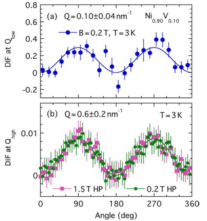
FIG. 10. Angle dependence of neutron response \text{DIF}(\theta) of \text{Ni}_{0.90}\text{V}_{0.10} for different Q ranges at low T = 3 K < T_c confirming magnetic response 2NM_x ; solid lines follow Eq. (6). (a) Low Q range covers (0.06-0.14) \text{ nm}^{-1} ; (b) high Q range includes (0.4-0.8) \text{ nm}^{-1} . HP denotes half-polarized data, where \text{DIF} = \text{D-U} .
