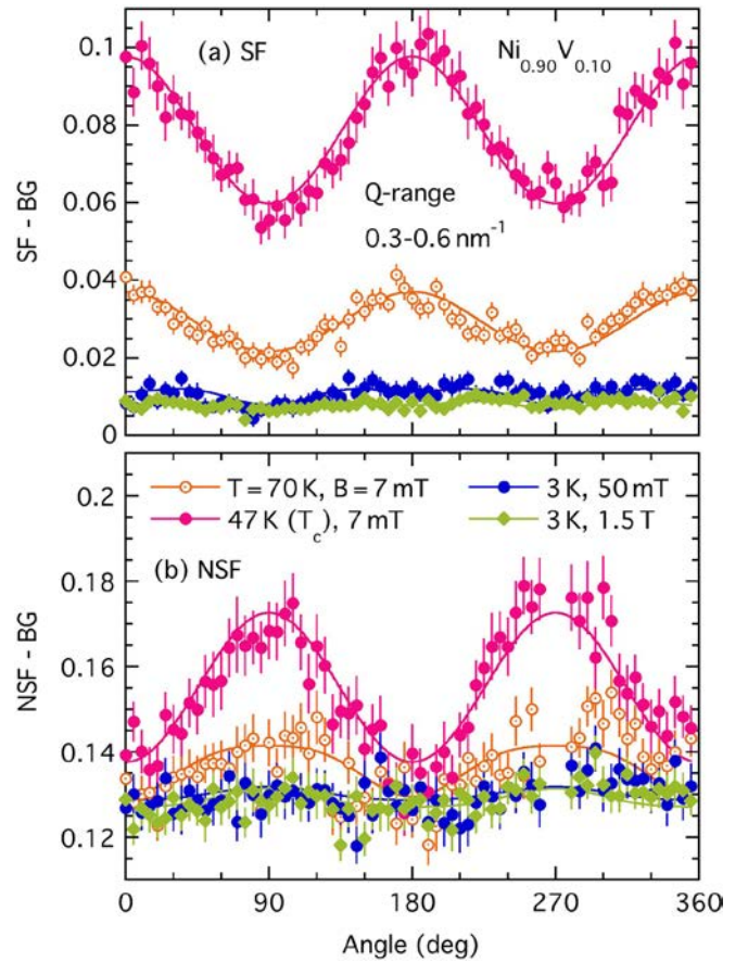
FIG. 3. Neutron scattering intensity of \text{Ni}_{0.90}\text{V}_{0.10} vs azimuthal angle \theta collected in medium Q range of (0.3-0.6) \text{ nm}^{-1} at different temperatures T and magnetic fields B . The upper panel (a) presents the SF data, the lower panel (b) the NSF data with fit as solid line using Eq. (1) in (a) and Eq. (4) in (b). An angle-independent background BG has been subtracted from the data, which varies with spin filter and B .
