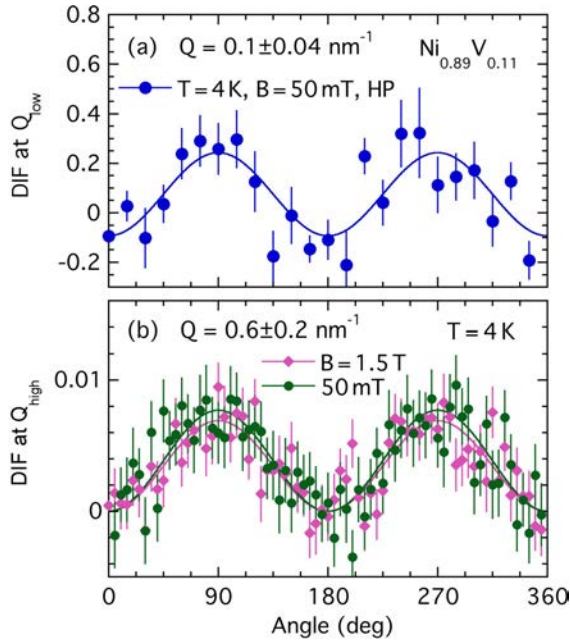
FIG. 13. Angle dependence of \text{DIF}(\theta) of \text{Ni}_{0.89}\text{V}_{0.11} for different Q ranges at low T = 4 \text{ K} < T_c confirming magnetic response 2NM_x ; solid lines follow Eq. (6) with a small offset. (a) Low Q range covers (0.06\text{--}0.14) \text{ nm}^{-1} ; (b) high Q range includes (0.4\text{--}0.8) \text{ nm}^{-1} . HP denotes half-polarized data, where \text{DIF} = \text{D-U} .
