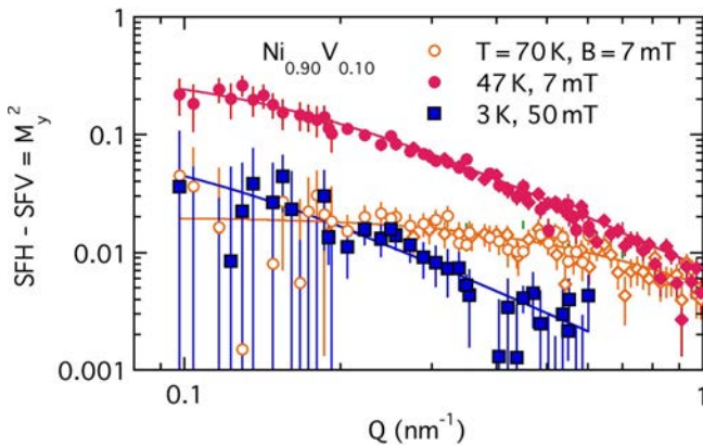
FIG. 5. Magnetic neutron scattering intensity vs wave vector Q for \text{Ni}_{0.90}\text{V}_{0.10} . The spin-flip contrast \text{SFH} - \text{SFV} is shown in small magnetic fields ( B \leq 50 mT) representing M_y^2 or 1/3 of the total isotropic magnetic response M_{\text{tot}}^2 for different temperatures T . Solid lines are Lorentzian fits using Eq. (7).
