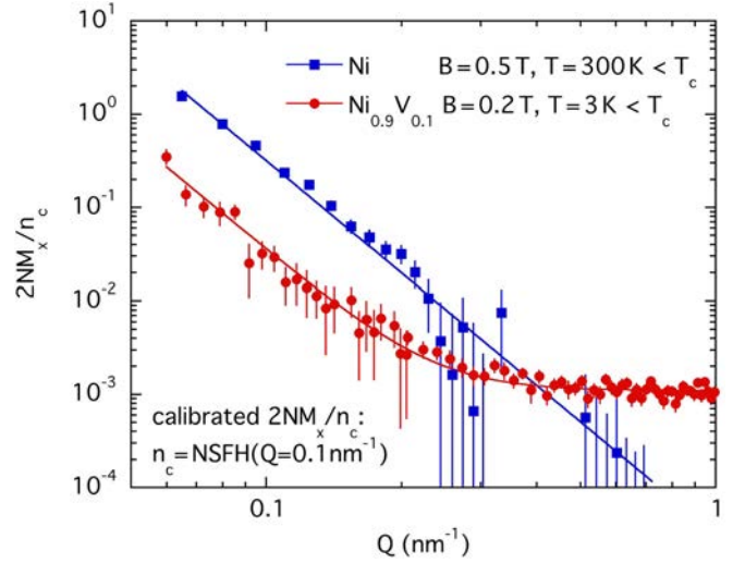
FIG. 16. Calibrated DIF response 2NM_x/n_c for Ni and \text{Ni}_{0.90}\text{V}_{0.10} vs wave vector Q . In Ni only the long-range ordered domain term is present; the local defects appear in the V alloy. The solid line is fit according to Eq. (8).
