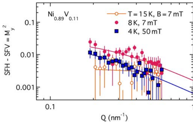
FIG. 7. Magnetic neutron scattering intensity vs wave vector Q for \text{Ni}_{0.89}\text{V}_{0.11} . The spin-flip contrast SFH-SFV is shown in small magnetic fields ( B \leq 50 mT) representing M_y^2 or 1/3 of the total isotropic magnetic response M_{\text{tot}}^2 for different temperatures T . Solid lines are Lorentzian fits using Eq. (7).
