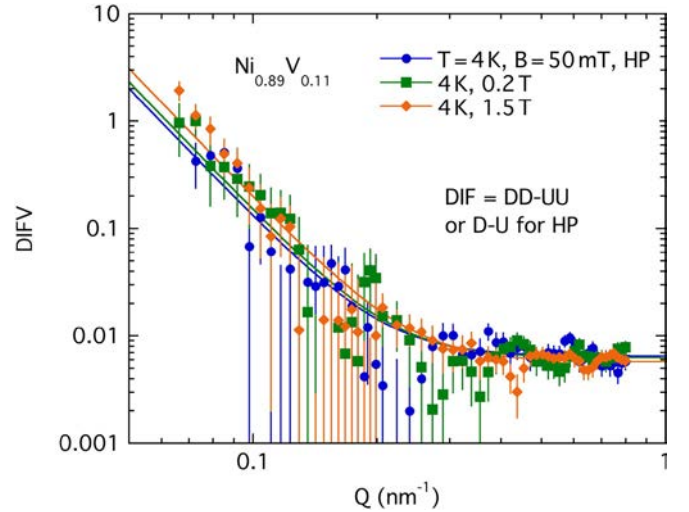
FIG. 14. Q dependence of \text{DIFV} = 2NM_x of \text{Ni}_{0.89}\text{V}_{0.11} at low T = 4 \text{ K} < T_c in magnetic fields B . Solid line indicates fit according to Eq. (8).
