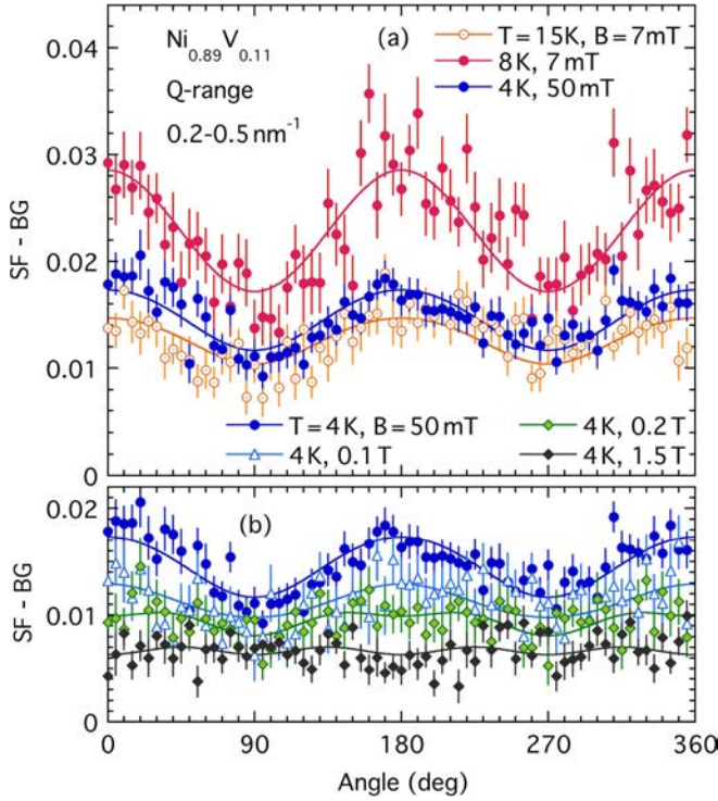
FIG. 6. Angle dependence of SF signal collected in medium Q range ( 0.35 \pm 0.15 ) \text{nm}^{-1} for \text{Ni}_{0.89}\text{V}_{0.11} . Panel (a) shows data in small magnetic fields B at different temperatures T , and panel (b) data at low T in different B . Fit is shown as solid line using Eq. (1). A constant BG has been subtracted from the data that depends on polarization filter and magnetic field.
