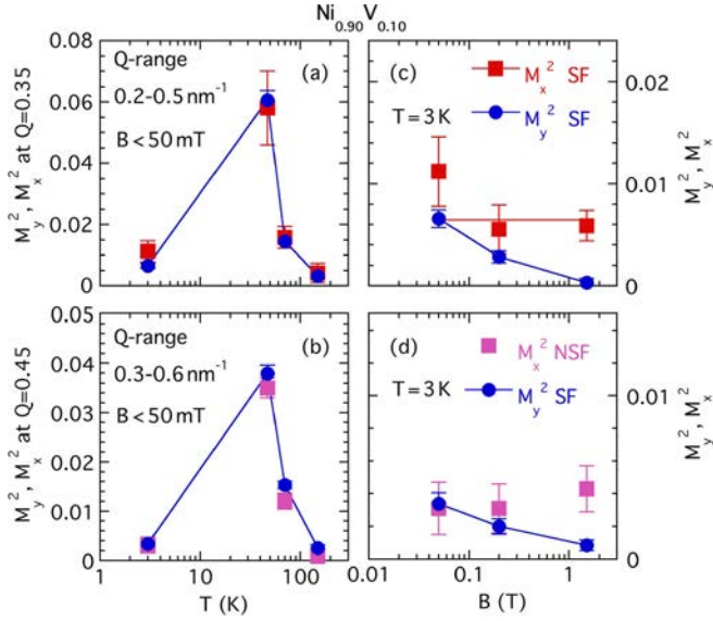
FIG. 4. Temperature T and magnetic field B dependence of magnetic transverse components M_y^2 and longitudinal component M_x^2 of \text{Ni}_{0.90}\text{V}_{0.10} . In the upper panel [(a), (c)] M_y^2 and M_x^2 are extracted from fit [Eq. (1)] of \text{SF}(\theta) at Q range (0.2–0.5) \text{nm}^{-1} . The lower panel [(b), (d)] presents the main components from the data shown in Fig. 3 at Q range (0.3–0.6) \text{nm}^{-1} : M_y^2 comes from fit of \text{SF}(\theta) and M_x^2 from fit [Eq. (4)] of \text{NSF}(\theta) .
