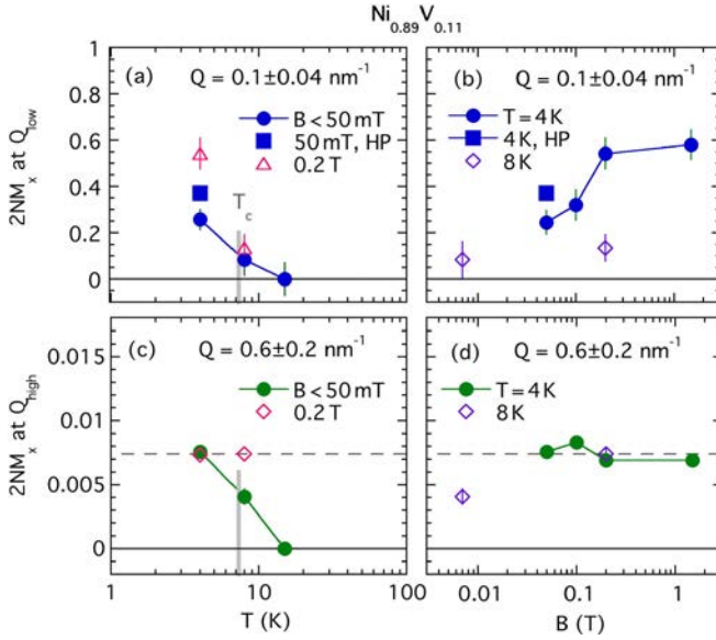
FIG. 15. Magnetic response 2NM_x of \text{Ni}_{0.89}\text{V}_{0.11} for low Q [upper panels (a), (b)] and high Q [lower panels (c), (d)] derived from \text{DIF}(\theta) . The left panels [(a), (c)] compare the temperature dependence in small magnetic fields as indicated ( B_{\text{low}} \leq 50 mT), the right panels [(b), (d)] the field dependence at T = 4 K < T_c and T = 8 K \approx T_c . While 2NM_x(Q_{\text{low}}) represents the ordered domain contribution, 2NM_x(Q_{\text{high}}) stems from local magnetic impurities.
