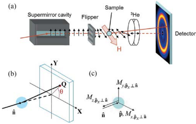
FIG. 2. (a) Polarized SANS setup with polarizing supermirror, spin flipper, sample in a cryostat with a magnetic field perpendicular to the neutron beam, a ^3\text{He} analyzer, and a position-sensitive detector. Arrows indicate neutron polarization direction. (b) Coordinate axes with beam direction \hat{n} along z defining angle \theta in the xy plane of the detector. (c) Present setup of field and polarization direction \hat{p} along x (from Ref. [36]).
