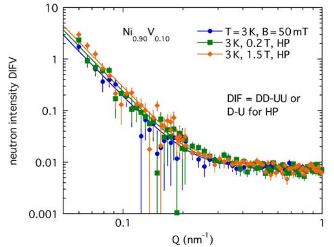
FIG. 11. Q dependence of \text{DIFV} = 2NM_x of \text{Ni}_{0.90}\text{V}_{0.10} at low T = 3 K < T_c in magnetic fields B . Solid line indicates fit according to Eq. (8).
