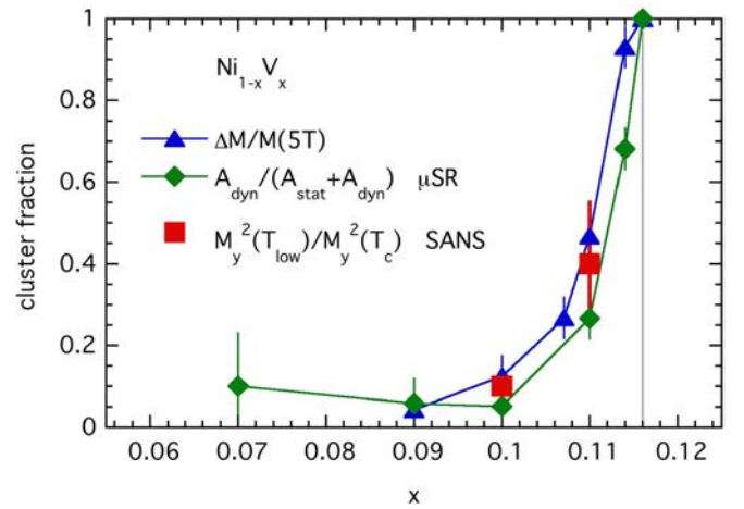
FIG. 18. Magnetic cluster fraction vs vanadium concentration x in \text{Ni}_{1-x}\text{V}_x obtained from SANS compared to other methods: magnetization M(B) , \mu\text{SR} from Ref. [26]. The SANS estimate is the ratio of the SF contrast at lowest T and T_c , taken in medium Q range.
