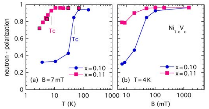
FIG. 19. Transmitted neutron beam polarization ratio P_s of the sample ( \text{Ni}_{0.90}\text{V}_{0.10} and \text{Ni}_{0.89}\text{V}_{0.11} ) at different environments. Panel (a) presents the temperature T dependence in a small field; both samples depolarize the beam for T < T_c . Panel (b) shows how the polarization recovers in applied magnetic fields B at a low temperature.
