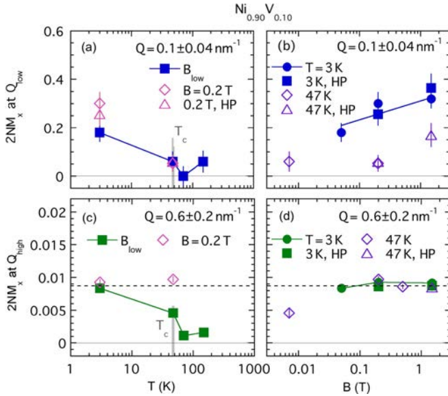
FIG. 12. Magnetic response 2NM_x of \text{Ni}_{0.90}\text{V}_{0.10} for low Q [upper panels (a), (b)] and high Q [lower panels (c), (d)] derived from \text{DIF}(\theta) . The left panels [(a), (c)] compare the temperature dependence in small magnetic fields as indicated ( B_{\text{low}} \leq 50 mT), the right panels [(b), (d)] the field dependence at T = 3 \text{ K} < T_c and T = 47 \text{ K} = T_c . While 2NM_x at Q_{\text{low}} represents the long-range magnetic domain contribution, 2NM_x at Q_{\text{high}} signals local magnetic impurities. The solid lines connect data points in (a), (c), (d).
