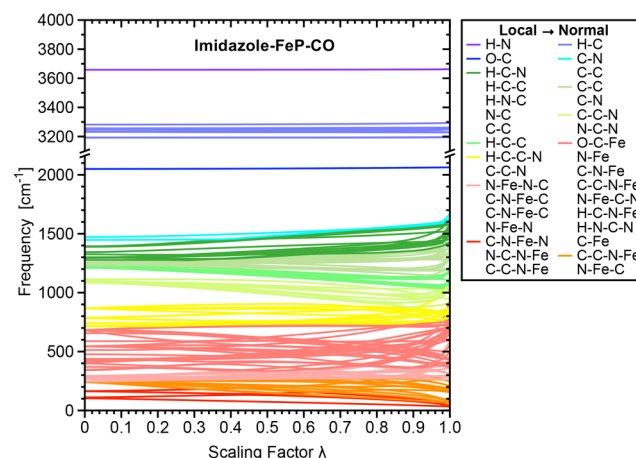
Figure 18. ACS plots of test example 10 (ligated Fe(II)-porphyrin L'–FeP–L, with L = CO, L' = imidazole) at the M06L/def2-TZVP level of theory relating local mode frequencies (left) with normal-mode frequencies (right). Local vibrational modes are indicated, while normal vibrational mode symmetries are suppressed.
