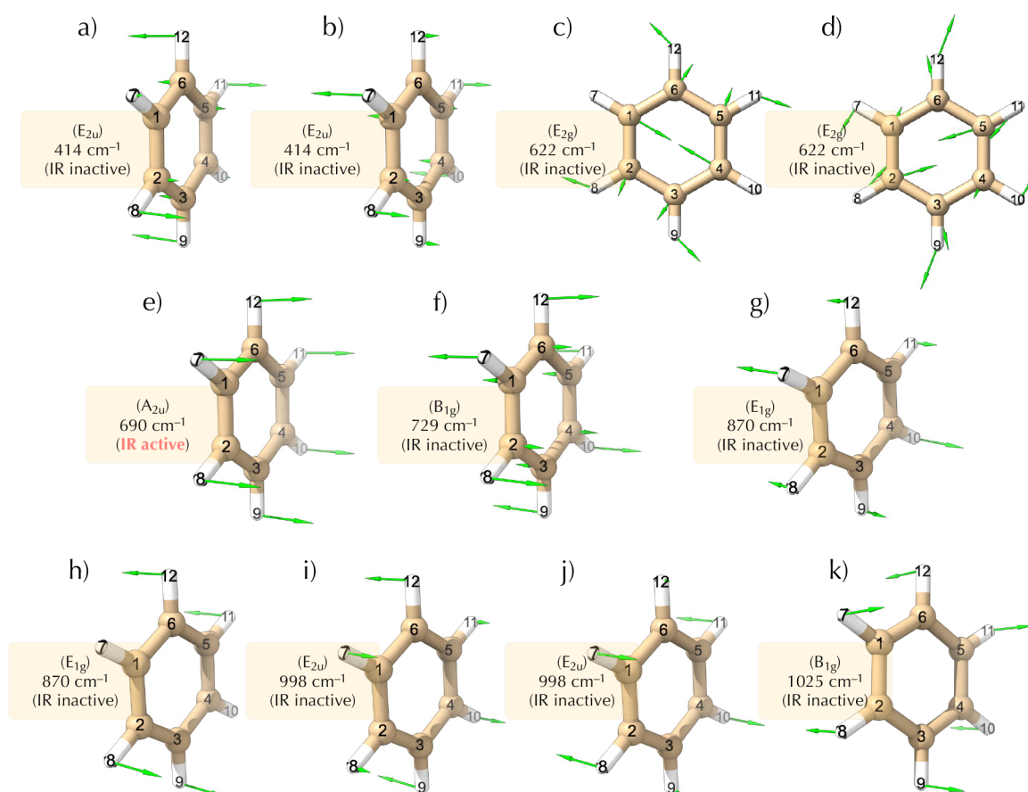
Figure 6. Displacement vectors for selected NVMs involving (a, b) C–C–C–C out-of-plane distortions; (c, d) C–C–C in-plane, and (e–h) C–C–C out-of-plane distortions for benzene in the D_{6h} point group obtained at the \omega B97X-D/aug-cc-pVDZ level of theory. Symmetry, normal-mode frequency \tilde{\nu} (in \text{cm}^{-1} ) and IR activity are indicated.
