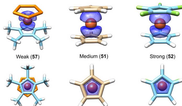
Fig. 9. The iso-surface of electron density for weak (57), medium (51), and strong (52) ferrocenes. The surface was generated using the independent gradient model 211 with the iso-surface value of 0.02.
