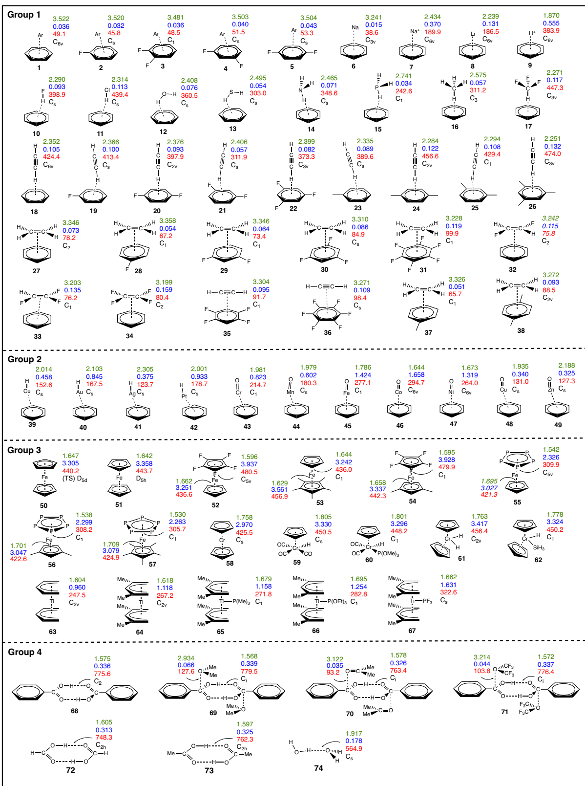
Fig. 1. Complexes investigated in this work. Intermonomer distances (Å) in green, corresponding local mode forces constants (mDyn/Å) in blue, and local mode frequencies (cm -1 ) in red. For a description of model chemistries used, see computational details.
