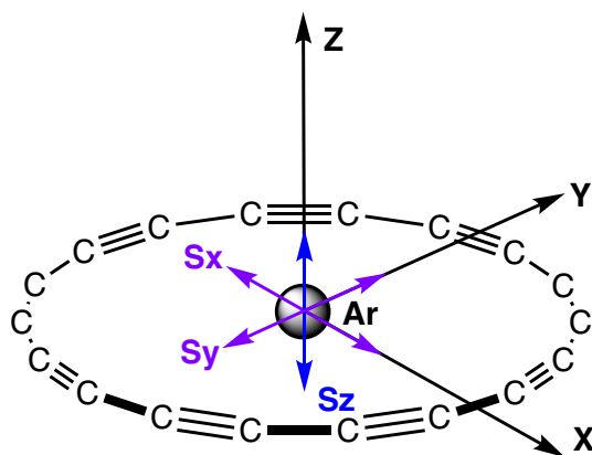
Fig. 3. Structure of planar Ar-C 18 complex. The S_z mode describing the out of plane motion of the Ar atom in blue color and S_x and S_y modes describing the in plane motion of the Ar atom in x and y directions, respectively, in purple color.
