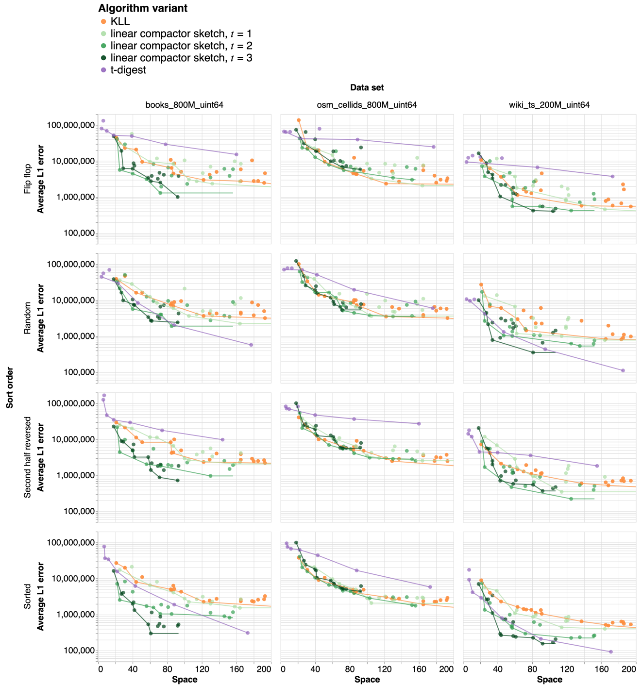
Figure 4: Space-error tradeoff curves for the baselines and linear compactor sketch on three different data sets from SOSD and four different sort order, described above. Markers indicate individual sketches, while curves indicate the lower frontier of possibilities observed (that is, the lower envelope described above) to highlight the general capabilities of each algorithm. A better algorithm has a curve that is further down and to the left, indicating lower error at a given amount of space.
