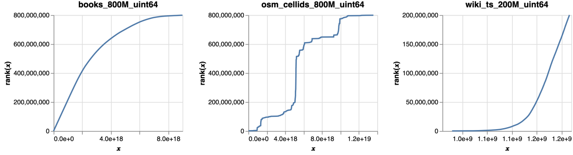
Figure 2: The rank functions for the three SOSD data sets used in our experiments. The three data sets have rank functions with distinctive shapes, allowing us to compare the algorithms in a variety of settings.
