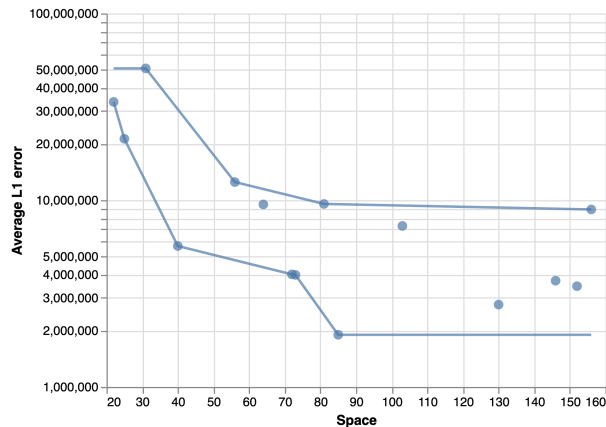
Figure 3: An example of the “envelope” or hull of the space-error data points for the linear compactor sketch with t = 2 ( books dataset, random order). It shows the range of errors that a user can expect from the linear compactor sketch given a certain amount of space.
