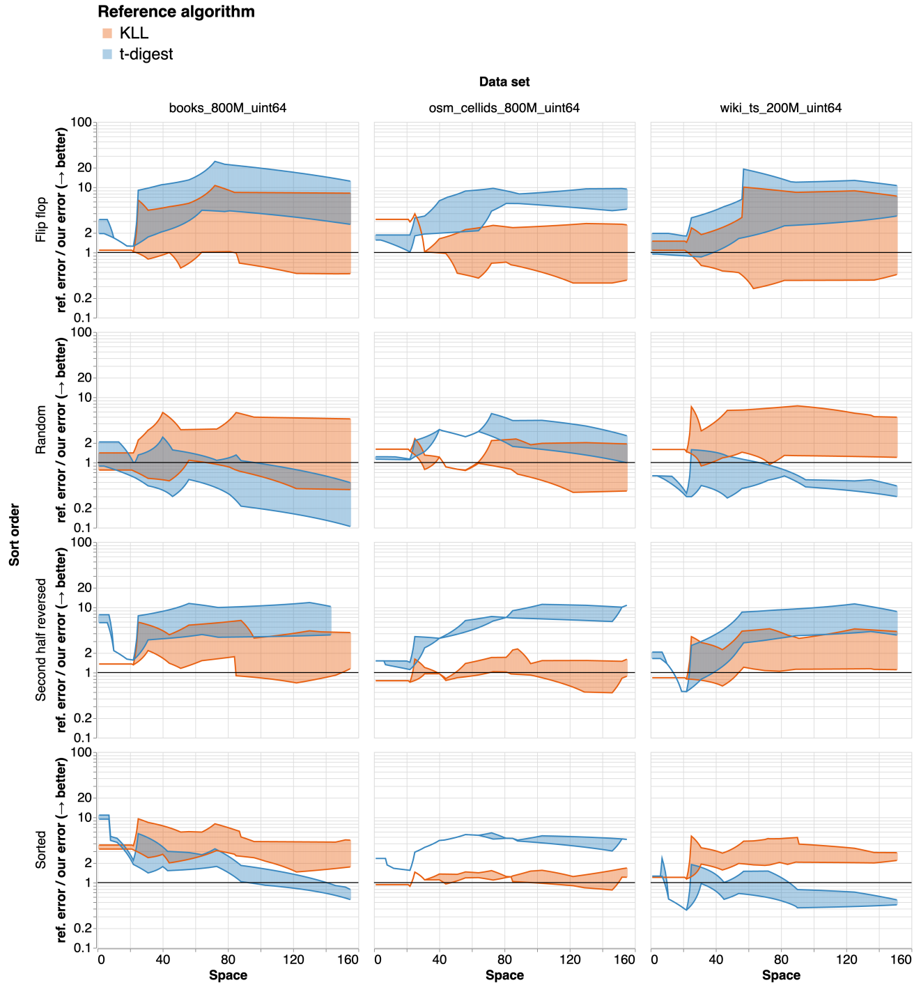
Figure 5: Hulls representing the possible ratios of the error achieved by a reference algorithm (either KLL or t-digest) to the error achieved by the linear compactor sketch with t = 2 . The filled-in area represents the area ratios consistent with the experiments in Figure 4. We see that the linear compactor sketch always achieve error no worse than 3\times that of KLL, while often achieving an error that is competitive with—and sometimes much lower than—that achieved by the t-digest.
