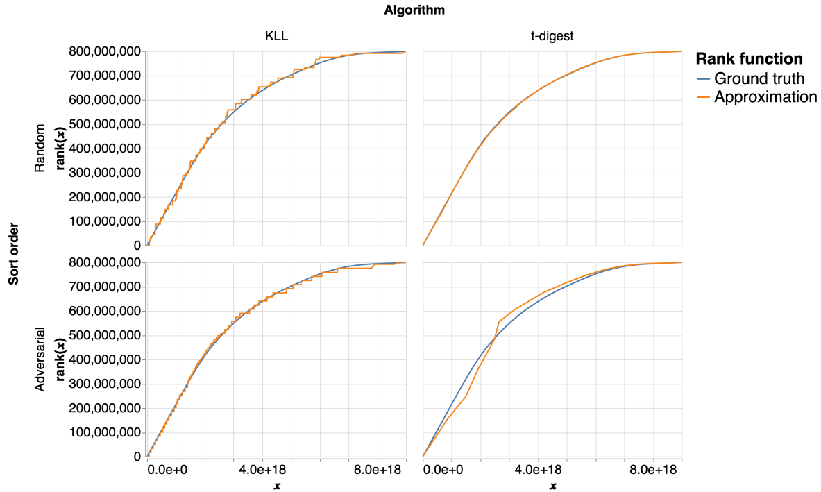
Figure 1: Ground-truth and approximate rank functions for the SOSD books data set, with approximation by both the KLL and t-digest sketches. For the approximations, the data were presented in both randomly shuffled (top) and adversarial (bottom) order. In the adversarial case that we discovered, t-digest does much worse than KLL, demonstrating the value of worst-case correctness.
