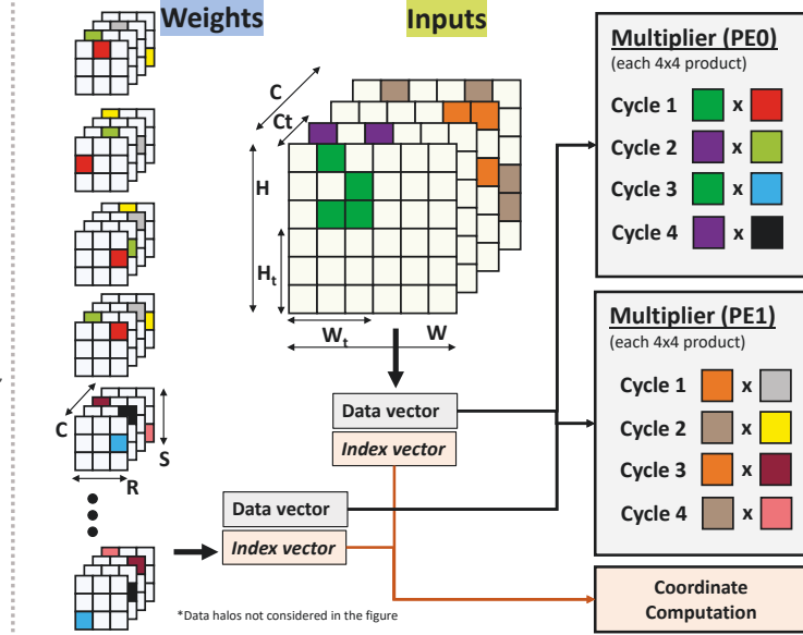
Figure 4: Code and example of proposed dataflow with higher temporal locality. In each cycle for multipliers PE0, PE1, operands in left denote values from input activations, and operands in right denote values from weights.
