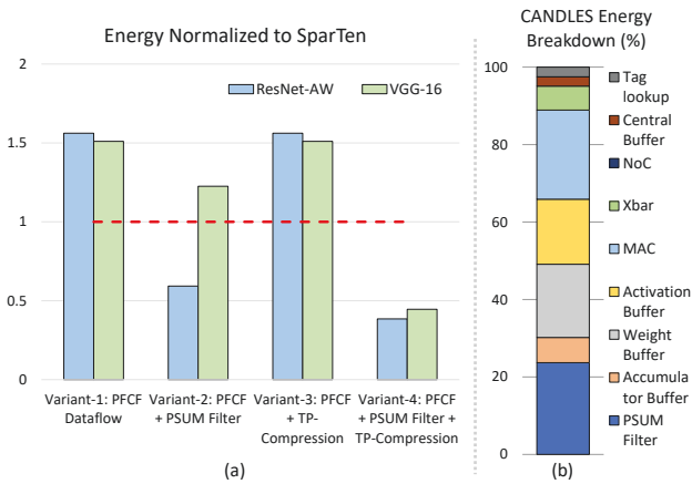
Figure 7: Energy breakdown in CANDLES .
