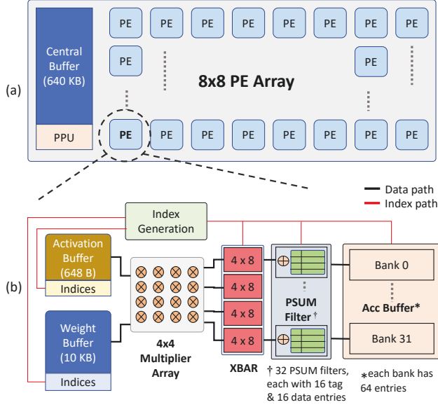
Figure 3: CANDLES Microarchitecture.
