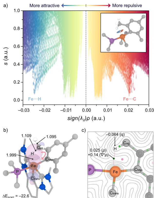
Fig. 2 (a) NCI plot for 1-PMe 3 , representing the reduced density gradient, s , as a function of the electron density \rho multiplied by the sign of the second eigenvalue of the Hessian matrix, \text{sign}(\lambda_2)\rho , which effectively displays NCIs as distinct peaks (see ESI† for more details). Colder/warmer colors depict attractive/repulsive interactions. Isosurfaces (isovalue = 0.3 a.u.) for the most relevant interactions are shown in the inset. (b) Selected donor–acceptor NBO interaction (isovalue = 0.07 a.u.) for 1-PMe 3 . The \Delta E_{\text{SOPT}} value (in kcal mol −1 ) and relevant distances (in Å) are provided. Most H atoms have been omitted, while the chelating ligand has been simplified for clarity. (c) Electron density map along the Fe···H–C plane obtained by QTAIM. Green/pink dots denote bond/ring critical points, respectively. Values of the \rho(r) and \nabla^2\rho(r) at the Fe···H bond critical point, as well as the H agostic AIM charge ( q ), are also given in a.u.
