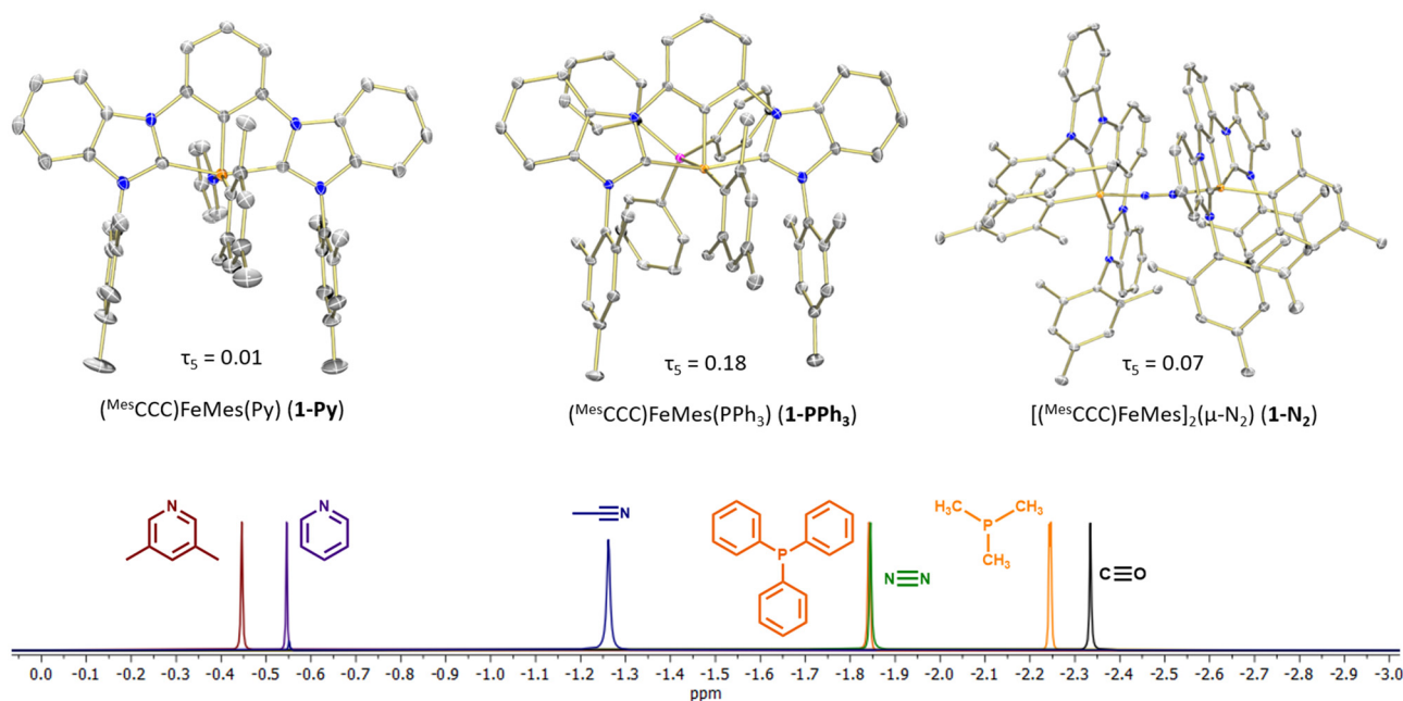
Fig. 1 Top panel: Molecular structures of 1-L (L = Py, PPh 3 and N 2 ) with 50% probability ellipsoids. Solvent molecules and hydrogen atoms have been omitted for clarity. Bottom panel: 1 H NMR spectral overlay of the agostic signal in 1-L complexes using benzene- d 6 as solvent.
