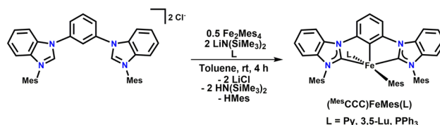
Scheme 1 Synthesis of 1-Py , 1-Lu , and 1-PPh 3 .
