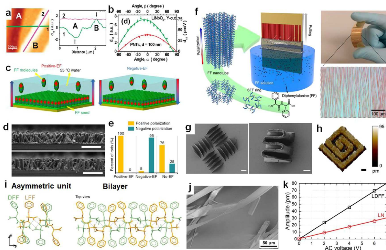
Figure 4. Piezoelectric peptides. (a) PFM image and d_{33} distribution in two directions indicating opposite piezoelectric polarizations of two FF nanotubes. (b) In-plane piezoresponse angle dependence for PNTs and Y-cut \text{LiNbO}_3 . Reprinted with permission from ref 65. Copyright 2010 American Chemical Society. (c) Illustration of FF microrods alignment under opposite electric field. (d) Cross-sectional SEM images of FF arrays under positive (up) and negative (bottom) electrical field (scale bars: 100 \mu\text{m} ). (e) Statistics of polarization directions of FF microrods under positive, negative, and no electrical field. Reprinted with permission under a Creative Commons CC BY License from ref 43. Copyright 2016 Springer Nature. (f) Illustration of aligned FF nanotubes growth by Meniscus-driven dip-coating method. Digital photograph and optical microscopy image of FF nanotube array on a flexible substrate. Reprinted with permission from ref 78. Copyright 2018 American Chemical Society. (g) Field-emission scanning electron microscopy images of 3D-printed FF microstructures. An array of microwalls with an isosceles trapezoid shape (scale bar: 20 \mu\text{m} ) and a zigzag wall (scale bar: 5 \mu\text{m} ). (h) 3D PFM image of an after-annealed FF spiral pattern (scale bar: 3 \mu\text{m} ). Reprinted with permission from ref 79. Copyright 2021 American Chemical Society. (i) The crystal structure of LDFF. (j) SEM image the LDFF tape. (k) Piezoresponse amplitude as a function of AC voltage of LDFF and lithium niobate (LN). Reprinted with permission from ref 80. Copyright 2021 John Wiley and Sons.
