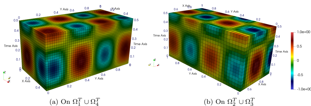
FIG. 8.1. Example 1, pressure computed with bilinear mortars on the space-time grid, refinement 3.
