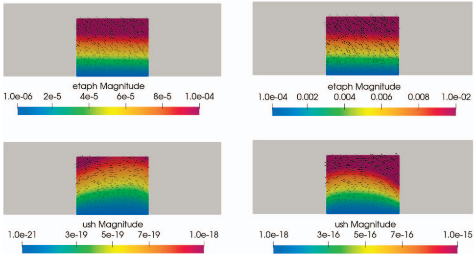
FIG. 9. Computed displacement \eta_{ph} and structure velocity \mathbf{u}_{sh} for the hard material (left) and soft material (right) at time T = 80 s. Top: displacement (arrows) and its magnitude (color); bottom: structure velocity (arrows) and its magnitude (color). (For interpretation of the colors in the figure(s), the reader is referred to the web version of this article.)
