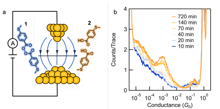
Figure 1. (a) Schematic representation of the electric field catalyzed homolysis of 4-(methylthio)benzoic peroxyanhydride 1 to yield 4-(methylthio)benzoic acid 2 . Blue arrows represent the electric field. (b) Logarithmically binned 1D histograms of consecutive conductance traces measured at different reaction times.
