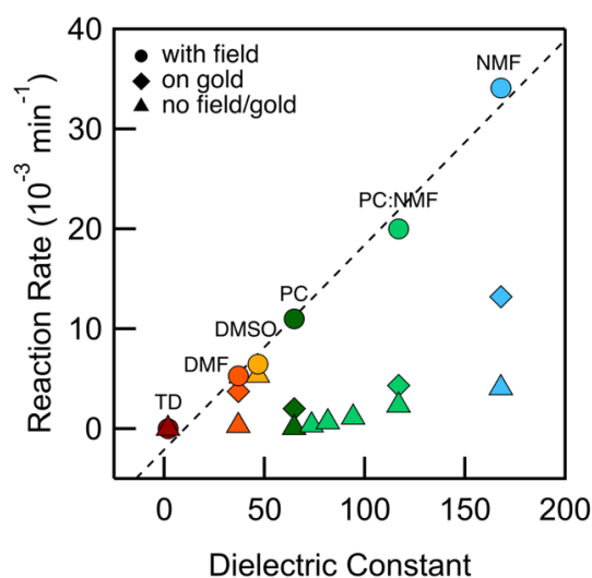
Figure 3. Rate of consumption of 1 in TD (dark red), DMF (orange), DMSO (yellow), PC (dark green), NMF (blue), and mixtures of PC and NMF (light green) in ratios of 1:10, 2:10, 4:10, 1:1 (from left to right) plotted against solvent dielectric. Data for rates are measured from STM-BJ measurements using an applied bias of 100 mV (circles), exposure to gold (diamonds) and without an applied field or exposure to gold (triangles). The dashed line is a linear fit to the data.
