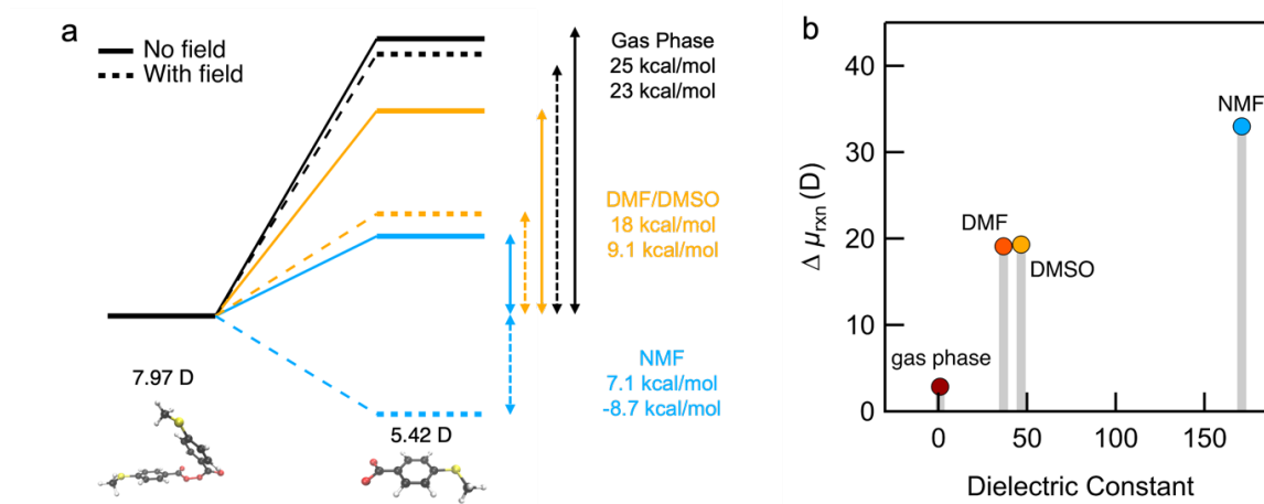
Figure 4. (a) Optimized geometries of reactant 1 and aroyloxy radical product indicating the gas phase dipole moments. Also shown are BDE in the gas phase and in different solvents, without a field (solid) and with a 1 V/nm field (dashed). (b) Computed dipole moment difference of 1 and aroyloxy radicals ( \Delta\mu_{\text{rxn}} = 2 \times \mu_{\text{aroyloxy radical}} - \mu_{\text{peroxide}} ) simulated in the gas phase, and in DMF, DMSO, and NMF using an implicit solvation model.
