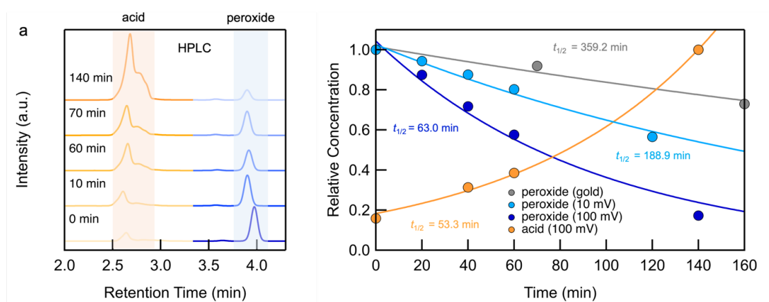
Figure 2. (a) HPLC chromatograms at 280 nm detection wavelength extracted from the STM-BJ solution at the times indicated. The peak for 2 shows some concentration dependent tailing, which likely arises from the formation of hydrogen bonded aggregates determined based on injections of pure 2 . (b) Relative concentration versus time of 2 at 100 mV (orange, reaction rate = 0.012 \pm 0.001 \text{ min}^{-1} ), 1 at 100 mV (dark blue, reaction rate = 0.011 \pm 0.001 \text{ min}^{-1} ), 1 at 10 mV (light blue, reaction rate = 0.0046 \pm 0.0004 \text{ min}^{-1} ) 1 without field (grey, reaction rate = 0.0019 \pm 0.0004 \text{ min}^{-1} ). The slow formation of 2 at 10 mV and without field was not measurable due to the changes in concentration being below detection limit.
