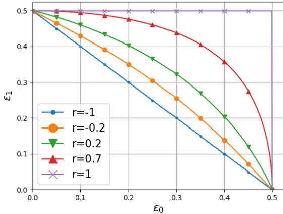
Fig. 1: \varepsilon_0 and \varepsilon_1 for a fixed 1 - F(\varepsilon_0, \varepsilon_1)
