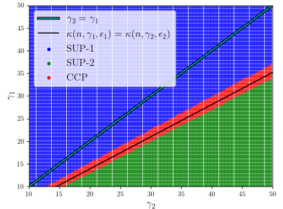
Fig. 3: Superior coding schemes for non-equal reliability
