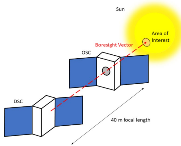
Figure 1. Conceptual depiction of VISORS distributed telescope formation geometry. 1
