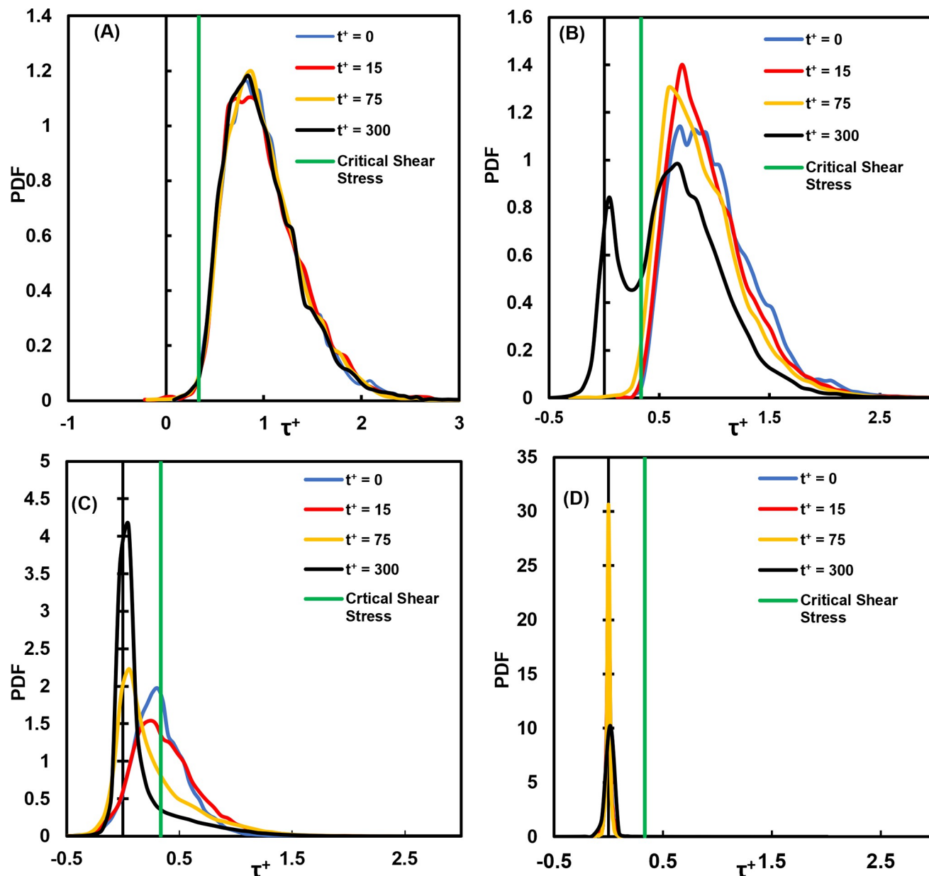
Fig 11. Distributions of shear stress on vWF particles at different times in viscous wall units. (A) Cloud released at the channel bottom wall, (B) release within the viscous sublayer ( Y_o = 1.5 ), (C) release within the buffer region ( Y_o = 15 ) and (D) release at the channel center.
