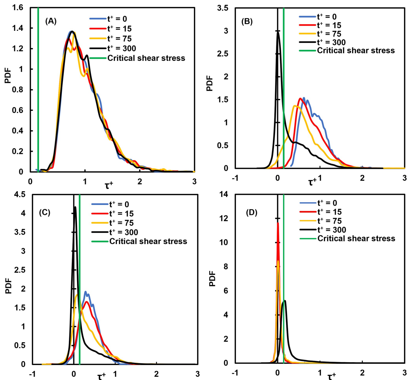
Fig 5. Distributions of shear stress on vWF particles at different times in viscous wall units. (A) Cloud released at the channel bottom wall, (B) release at the edge of the viscous wall subregion ( Y_0 = 5 ), (C) release within the buffer region ( Y_0 = 15 ) and (D) release at the channel center.
