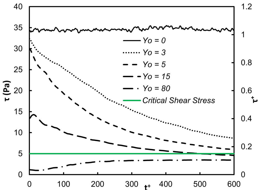
Fig 4. Average of actual shear stresses. The abscissa in dimensionless viscous parameters and in dimensional units is shown. One can adjust the dimensional stress axis at the same Re by considering a new channel width with a new corresponding mean velocity to recalculate \tau_w and u^* , and using the dimensionless values presented.
