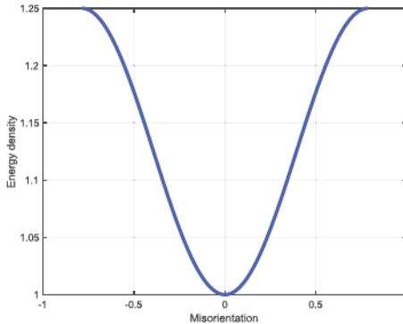
Fig. 3. Grain boundary energy density function \sigma(\Delta\alpha) .
