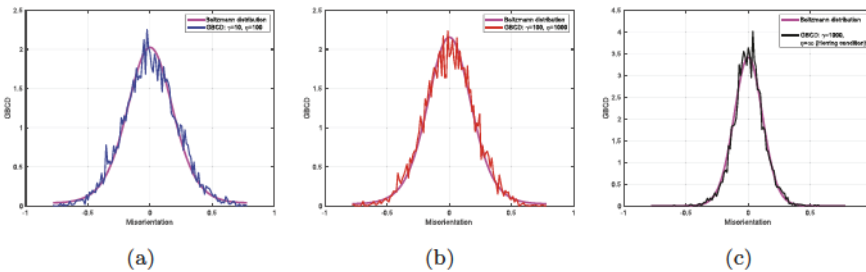
Fig. 9. (Color online) Grain growth system (5.2) with finite \mu (with curvature), one run of 2D trial with 10,000 initial grains: (a) Left plot, GBCD (blue curve) at T_\infty versus Boltzmann distribution with “temperature” — D \approx 0.064 (magenta curve), grain growth system with mobility of triple junctions \eta = 100 and the misorientation parameter \gamma = 10 . (b) Middle plot, GBCD (red curve) at T_\infty versus Boltzmann distribution with “temperature” — D \approx 0.058 (magenta curve), grain growth system with mobility of triple junctions \eta = 1000 and the misorientation parameter \gamma = 100 . (c) Right plot, GBCD (black curve) at T_\infty versus Boltzmann distribution with “temperature” — D \approx 0.026 (magenta curve), grain growth system with mobility of triple junctions \eta \rightarrow \infty (Herring condition) and the misorientation parameter \gamma = 1000 .
