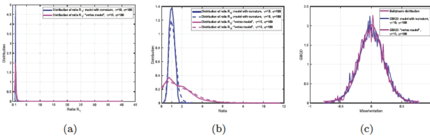
Fig. 13. (Color online) One run of 2D trial with 10,000 initial grains: (a) Left plot: Comparison of distributions of ratio R_1 (5.3) (solid blue) for model with curvature (finite \mu ) (5.2) and R_1 (5.3) (solid magenta) “vertex model” with ( \mu \rightarrow \infty ) (5.2). (b) Middle plot: comparison of distributions of ratio R_2 (5.4) (solid blue) and R_3 (5.5) (dashed blue) for model with curvature (finite \mu ) (5.2), and comparison of distributions of ratio R_2 (5.4) (solid magenta) and R_3 (5.5) (dashed magenta) for “vertex model” with ( \mu \rightarrow \infty ) (5.2). The distributions are plotted at T_\infty . (c) Right plot: One run of 2D trial with 10,000 initial grains, GBCD (blue curve) “curvature model” (finite \mu ) (5.2), GBCD (dark magenta curve) “vertex model” ( \mu \rightarrow \infty ) (5.2) at T_\infty versus Boltzmann distribution with “temperature” — D \approx 0.064 (magenta curve). Grain growth “curvature model” is considered with mobility of triple junctions \eta = 100 and \gamma = 10 , and grain growth “vertex model” is considered with mobility of triple junctions \eta = 100 and \gamma = 15 .
