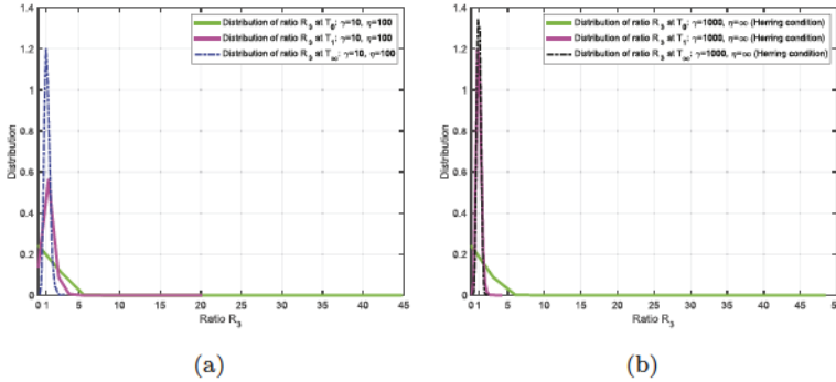
Fig. 8. (Color online) Grain growth system (5.2) with finite \mu (with curvature), one run of 2D trial with 10,000 initial grains: (a) Left plot, distributions of ratio R_3 (5.5) at initial time T_0 (solid green), at a time T_1 after a first time step (solid magenta) and at a final time T_\infty (dashed point blue) for grain growth system with mobility of triple junctions \eta = 100 and the misorientation parameter \gamma = 10 . (b) Right plot, distributions of ratio R_3 (5.5) at initial time T_0 (solid green), at a time T_1 after a first time step (solid magenta) and at a final time T_\infty (dashed point black) for grain growth system with mobility of triple junctions \eta \rightarrow \infty (Herring condition) and the misorientation parameter \gamma = 1000 . The closest mesh node of the grain boundary to the triple junction a is used as x_i .
