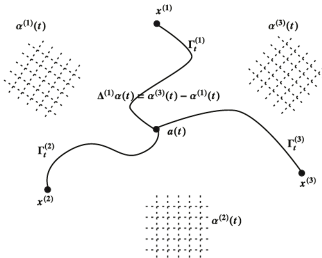
Fig. 1. Grain boundaries/curves \Gamma_t^{(j)} that meet at a triple junction \mathbf{a}(t) . Lattice orientations are angles (scalars) \alpha^{(j)}(t) . Misorientation \Delta^{(j)}\alpha(t) of \Gamma_t^{(j)} is the difference between two lattice orientations of grains that share grain boundary \Gamma_t^{(j)} .
