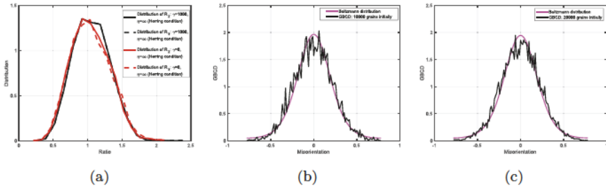
Fig. 11. (Color online) Grain growth system (5.2) with finite \mu (with curvature): (a) Left plot, one run of 2D trial with 10,000 initial grains, comparison of distributions of ratio R_2 (5.4) (solid black) and R_3 (5.5) (dashed black), grain growth system with mobility of triple junctions \eta \rightarrow \infty (Herring condition) and \gamma = 1000 . Comparison of distributions of ratio R_2 (5.4) (solid red) and R_3 (5.5) (dashed red), grain growth system with mobility of triple junctions \eta \rightarrow \infty (Herring condition) and no dynamic misorientations ( \gamma = 0 ). The closest mesh node of the grain boundary to the triple junction a is used as x_i . The distributions are plotted at T_\infty . (b) Middle plot, one run of 2D trial with 10,000 initial grains, GBCD (black curve) at T_\infty versus Boltzmann distribution with “temperature” — D \approx 0.068 (magenta curve). (c) Right plot, one run of 2D trial with 20,000 initial grains, GBCD (black curve) at T_\infty versus Boltzmann distribution with “temperature” — D \approx 0.069 (magenta curve). Grain growth system with mobility of triple junctions \eta \rightarrow \infty (Herring condition) and no dynamic misorientation ( \gamma = 0 ).
