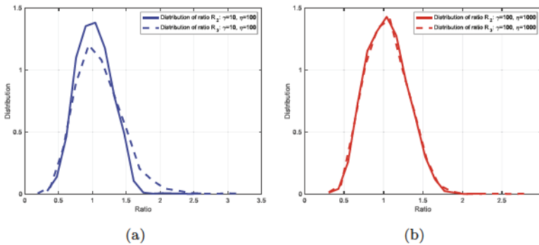
Fig. 5. (Color online) Grain growth system (5.2) with finite \mu (with curvature), one run of 2D trial with 10,000 initial grains: (a) Left plot, comparison of distributions of ratio R_2 (5.4) (solid blue) and R_3 (5.5) (dashed blue) for grain growth system with mobility of triple junctions \eta = 100 and the misorientation parameter \gamma = 10 . (b) Right plot, comparison of distributions of ratio R_2 (5.4) (solid red) and R_3 (5.5) (dashed red) for grain growth system with mobility of triple junctions \eta = 1000 and the misorientation parameter \gamma = 100 . The closest mesh node of the grain boundary to the triple junction \alpha is used as x_i . The distributions are plotted at T_\infty .
