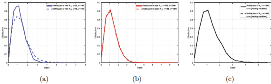
Fig. 7. (Color online) Grain growth system (5.2) with finite \mu (with curvature), one run of 2D trial with 10,000 initial grains: (a) Left plot, comparison of distributions of ratio R_2 (5.4) (solid blue) and R_3 (5.5) (dashed blue) for grain growth system with mobility of triple junctions \eta = 100 and the misorientation parameter \gamma = 10 . (b) Middle plot, comparison of distributions of ratio R_2 (5.4) (solid red) and R_3 (5.5) (dashed red) for grain growth systems with mobility of triple junctions \eta = 1000 and the misorientation parameter \gamma = 100 . (c) Right plot, comparison of distributions of ratio R_2 (5.4) (solid black) and R_3 (5.5) (dashed black) for grain growth system with mobility of triple junctions \eta \rightarrow \infty and the misorientation parameter \gamma = 1000 . The other triple junction (different from a) of the given grain boundary is used as x_i here. The distributions are plotted at T_\infty .
