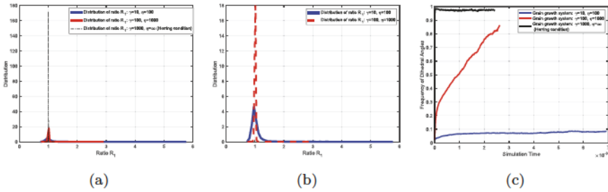
Fig. 4. (Color online) Grain growth system (5.2) with finite \mu (with curvature), one run of 2D trial with 10,000 initial grains: (a) Left plot, distribution of ratio R_1 (5.3) for grain growth systems with mobility of triple junctions \eta = 100 and the misorientation parameter \gamma = 10 (solid blue), with mobility of triple junctions \eta = 1000 and the misorientation parameter \gamma = 100 (solid red) and with mobility of triple junctions \eta \rightarrow \infty (Herring condition) and the misorientation parameter \gamma = 1000 (dashed point black). (b) Middle plot, comparison of the two distributions of ratio R_1 (5.3) for grain growth systems with mobility of triple junctions \eta = 100 and the misorientation parameter \gamma = 10 (solid blue) and with mobility of triple junctions \eta = 1000 and the misorientation parameter \gamma = 100 (dashed red). The distributions are plotted at T_\infty . (c) Right plot, time evolution of frequency of dihedral angles that satisfy ratio R_1 with 0.01 accuracy for grain growth systems with mobility of triple junctions \eta = 100 and the misorientation parameter \gamma = 10 (solid blue), with mobility of triple junctions \eta = 1000 and the misorientation parameter \gamma = 100 (solid red) and with mobility of triple junctions \eta \rightarrow \infty (Herring condition) and the misorientation parameter \gamma = 1000 (solid black).
