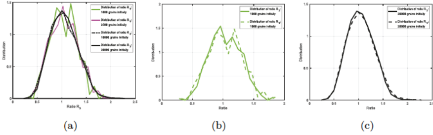
Fig. 10. (Color online) Grain growth system (5.2) with finite \mu (with curvature): (a) Left plot, distributions of ratio R_3 (5.5) system with 1000 grains initially (solid green), system with 2500 grains initially (solid magenta), system with 10,000 grains initially (dashed point black), and system with 20,000 grains initially (solid black). (b) Middle plot, comparison of distributions of ratio R_2 (5.4) (solid green) and R_3 (5.5) (dashed green) for system with 1000 grains initially. (c) Right plot, comparison of distributions of ratio R_2 (5.4) (solid black) and R_3 (5.5) (dashed black) system with 20,000 grains initially. Grain growth systems are considered with mobility of triple junctions \eta \rightarrow \infty (Herring condition) and no dynamic misorientation ( \gamma = 0 ). The closest mesh node of the grain boundary to the triple junction a is used as x_i . The distributions are plotted at T_\infty .
