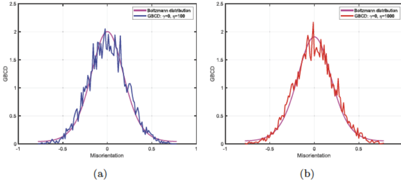
Fig. 12. (Color online) Grain growth system (5.2) with finite \mu (with curvature), one run of 2D trial with 10,000 initial grains: (a) Left plot, GBCD (blue curve) at T_\infty versus Boltzmann distribution with “temperature” — D \approx 0.066 (magenta curve), grain growth system with mobility of triple junctions \eta = 100 and no dynamic misorientation ( \gamma = 0 ). (b) Right plot, GBCD (red curve) at T_\infty versus Boltzmann distribution with “temperature” — D \approx 0.071 (magenta curve), grain growth system with mobility of triple junctions \eta = 1000 and no dynamic misorientation ( \gamma = 0 ).
