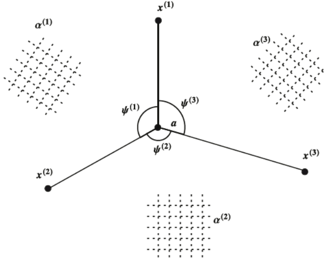
Fig. 2. The angles \psi_1, \psi_2, \psi_3 are defined as the above figure.
