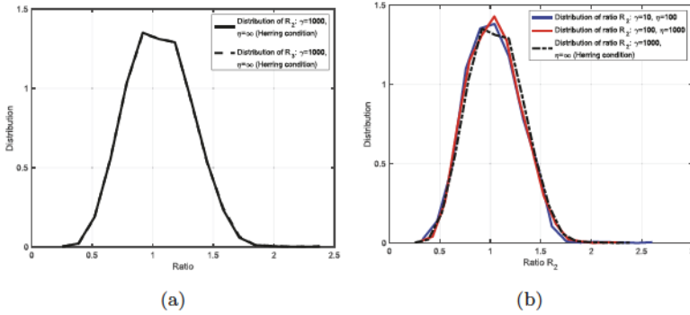
Fig. 6. (Color online) Grain growth system (5.2) with finite \mu (with curvature), one run of 2D trial with 10,000 initial grains: (a) Left plot, comparison of distributions of ratio R_2 (5.4) (solid black) and R_3 (5.5) (dashed black) for grain growth system with mobility of triple junctions \eta \rightarrow \infty (Herring condition) and the misorientation parameter \gamma = 1000 . (b) Right plot, comparison of distributions of ratio R_2 (5.4) for grain growth systems with mobility of triple junctions \eta = 100 and the misorientation parameter \gamma = 10 (solid blue), with mobility of triple junctions \eta = 1000 and the misorientation parameter \gamma = 100 (solid red), and with mobility of triple junctions \eta \rightarrow \infty (Herring condition) and the misorientation parameter \gamma = 1000 (dashed point black). The closest mesh node of the grain boundary to the triple junction a is used as x_i . The distributions are plotted at T_\infty .
