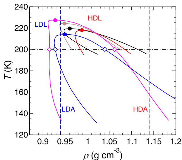
Fig. 1 | Comparison of estimates for the LDL–HDL binodal. Solid lines are binodals predicted from thermodynamic modeling of experimental data in ref. 11 (blue and brown), ref. 12 (magenta), and ref. 13 (black and red), with corresponding critical points marked by filled circles. Diamonds locate the coexistence densities of LDL and HDL at 200 K as determined by the magenta and blue binodals. Vertical dashed lines are isochores at the density of LDA (blue) and HDA (red) at T = 80 K and ambient pressure 22 . The dot-dashed line is an isotherm at 200 K.
