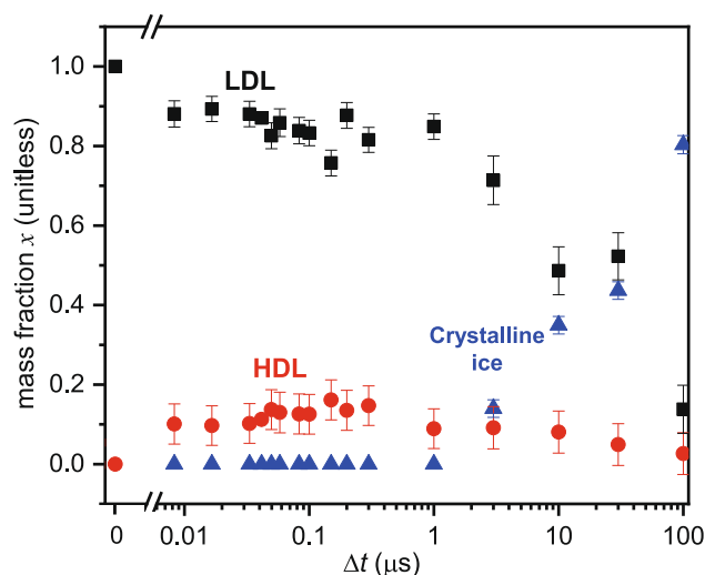
Fig. 4 | Time evolution of LDL, HDL and ice components after heating. Mass fraction of LDL (black squares), HDL (red circles), and crystalline ice (blue triangles) as a function of the pump-probe delay time \Delta t . Each data point is obtained by fitting our \Delta I(q) curves, averaged over three x-ray shots, to a sum of contributions due to LDA, HDA and crystalline ice, using the same procedure as described in ref. 8 . The error bars show the standard error for each data point determined by propagating the error associated with the averaged \Delta I(q) curves.
