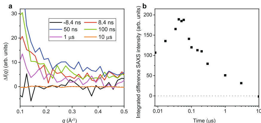
Fig. 5 | Small-angle x-ray scattering results. a The difference between the unpumped and pumped scattering curves at various time delays in the SAXS region. b Time-dependent integrated difference SAXS intensity from q = 0.1 to 0.3 \text{ \AA}^{-1} .
