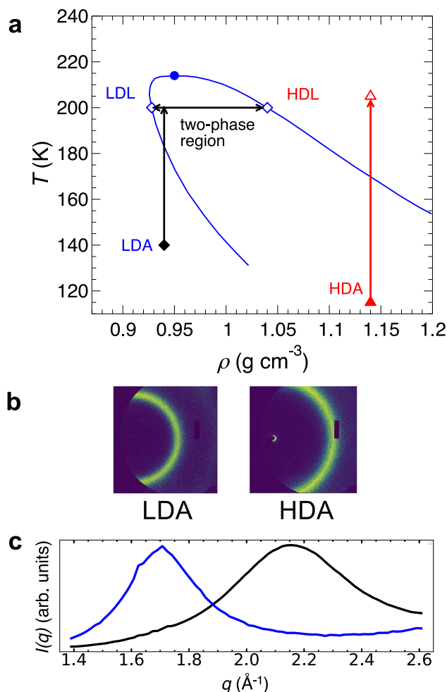
Fig. 2 | Isochoric heating of LDA to access the LDL-HDL coexistence region. a The blue curve is the binodal predicted from thermodynamic modeling in ref. 11 , with the corresponding critical point marked by the filled circle. The red arrow corresponds to an isochoric heating pathway, of the kind explored in ref. 8 , in which HDA (filled triangle) is heated to HDL (open triangle). The vertical black arrow illustrates the isochoric heating pathway explored here, in which LDA (filled diamond) is heated to a liquid state inside the two-phase region of the binodal. This state then phase separates into LDL and HDL components (horizontal arrows). Open diamonds locate the coexistence densities of LDL and HDL at 200 K as determined by the binodal. b, c Characteristic x-ray scattering intensities for LDA and HDA as observed ( b ) on the 2D experimental detector and ( c ) as I(q) scattering intensity curves as a function of wave number q . The LDA x-ray data shown in ( b, c ) is for the LDA sample prior to IR heating. The HDA x-ray data shown in ( b, c ) is for a HDA sample as reported in ref. 8 . I(q) for LDA and HDA is nearly identical to that for LDL and HDL, respectively 8,30 .
