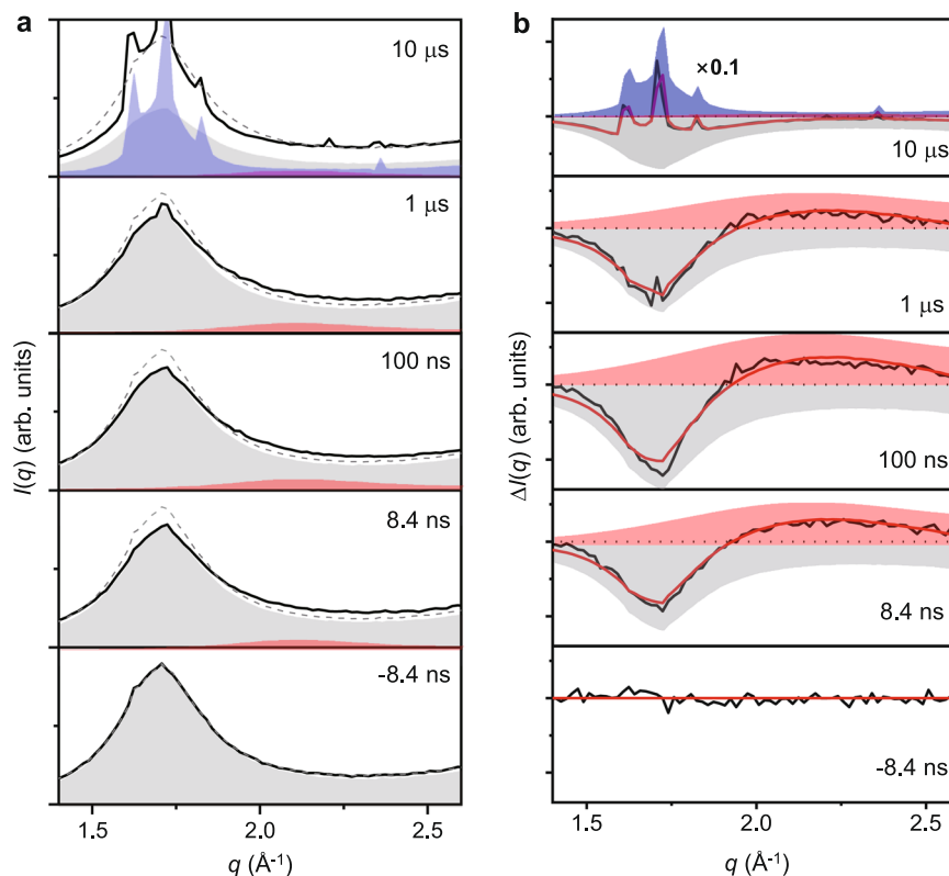
Fig. 3 | Structure factor before and after heating LDA. a Experimental x-ray scattering intensities, I(q) , of LDA samples measured before (gray dashed line) and after the laser excitation (black solid line). Data obtained at IR pump/x-ray probe delay times of \Delta t = -8.4 ns to 10 \mu s are shown. Each curve is obtained from the average of I(q) over three independent x-ray shots. The contributions from LDA, HDA, and crystalline ice are indicated as gray, red, and blue shaded areas,
