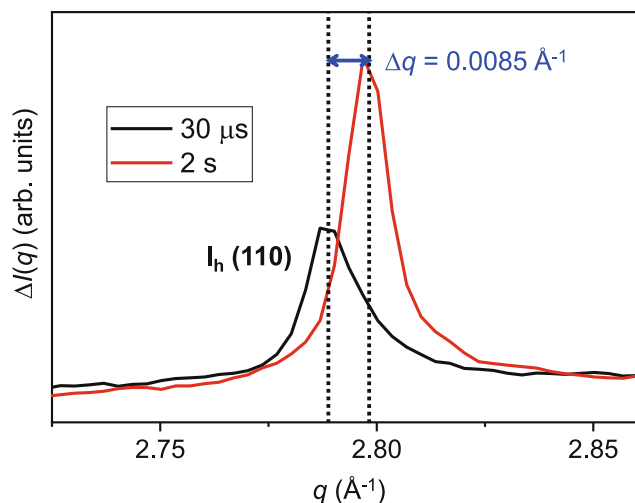
Fig. 6 | Bragg peak shift in ice following laser heating. Ice I_h (110) peak positions measured at 30 \mu s (black) and 2 s (red) after laser excitation of the sample. The shown peak shift of 0.0085 \text{\AA}^{-1} corresponds to a temperature difference of approximately 90 K in ice I_h . As described in the text, this temperature change implies that the temperature of the LDA sample was increased by 60 K by the IR laser pulse, prior to crystallizing.
