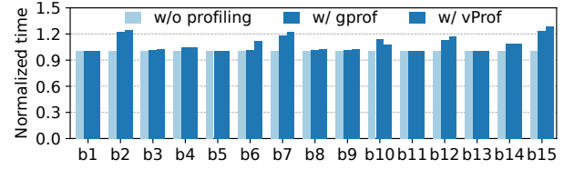
Figure 7. Profiling overhead for performance issues.
