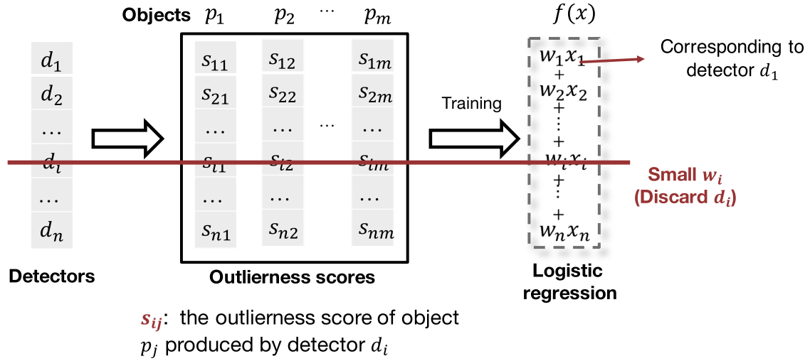
Fig. 2. AutoOD-Augment: Prune Poor Detectors
