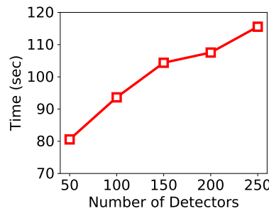
Fig. 6. Scalability on the Number of Detectors
