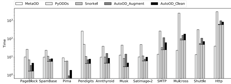
Fig. 5. Runtime Evaluation
