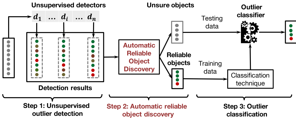
Fig. 1. AutoOD Framework
