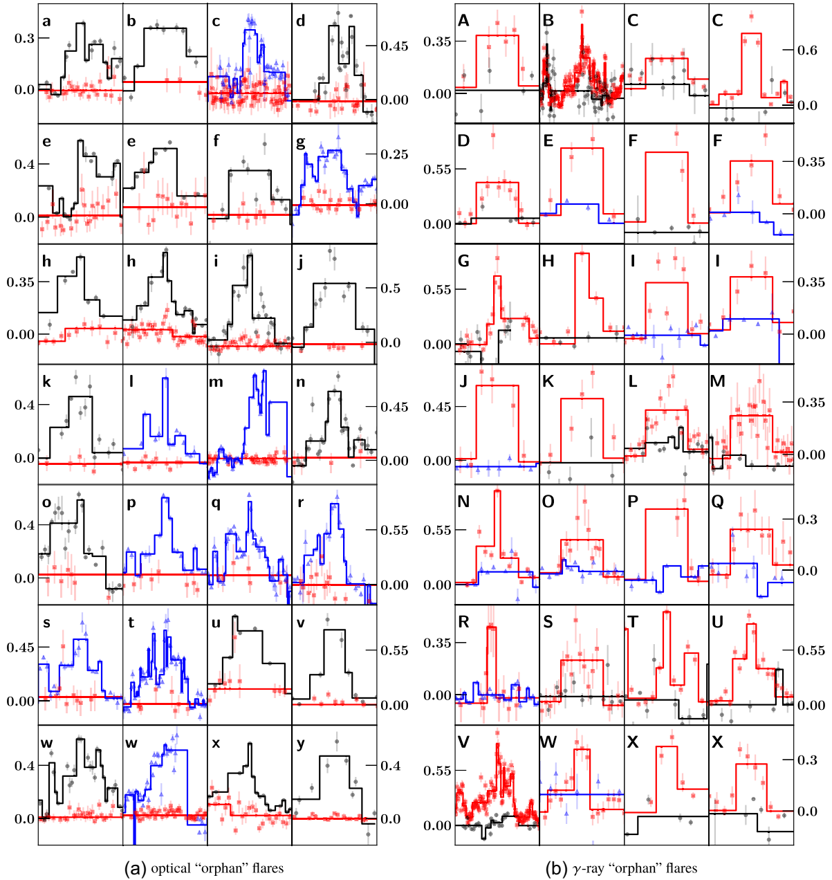
Figure 7. Gold sample of optical (left-hand panel) and \gamma -ray (right-hand panel) ‘orphan’ flares. The black dots, blue triangles, and red squares are optical V, optical g, and \gamma -ray fluxes, respectively. The letter in each panel corresponds to the blazar name in Table B1.
