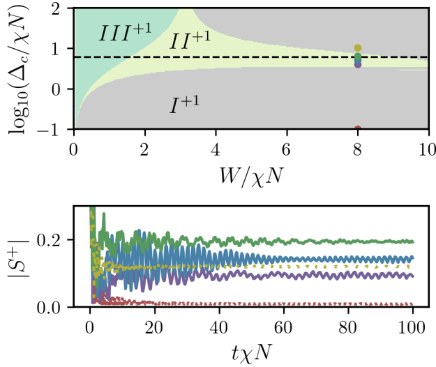
FIG. 3. Top panel: Dynamical phase diagram as a function of the cavity detuning and atomic disorder. The approximate resonance condition, \Delta_c \approx \epsilon_0 = 6\chi N , is marked by a black dashed line. Bottom panel: Dynamics of |S^+(t)| for W/(\chi N) = 8 and different values of \Delta_c/(\chi N) as marked by the points in the top panel. For \Delta_c/(\chi N) = 0.1 (red) and 10.3 (yellow), |S^+(t)| evolves to a constant steady state characteristic of phase I^{+1} , while for the remaining values of \Delta_c/(\chi N) , the dynamics have persistent oscillation characteristics of phase II^{+1} . In this figure, the initial state has \langle \hat{\sigma}_i^x \rangle = 1 and \langle a \rangle = 0 .
