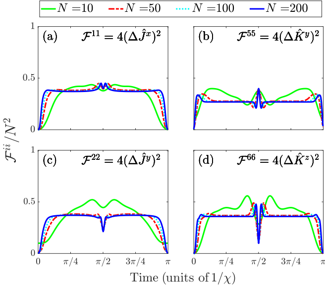
FIG. 2. Four of the six diagonal elements of the QFIM, for four different atom numbers. The operators \hat{J}^z and \hat{K}^x are left out because they commute with the Hamiltonian and are therefore conserved quantities. We see that as the number of atoms grows, the behavior of the diagonal QFIM elements converge. For atom numbers of N \approx 50 or more, a plateau with respect to time appears, centered around \chi t = \pi/4 . This is similar to the behavior found in OAT where the QFIM for \hat{J}^x and \hat{J}^y reaches a plateau [5] centered around the same time. As N grows, the plateau exists almost everywhere in time. Here we only show even atom numbers, N , but we note that for odd atom numbers the behavior is the same except for at \chi t = \pi/2 , where the concavity is opposite from what is shown here.
