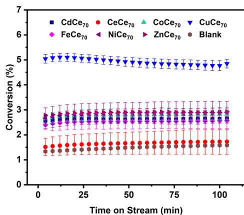
Figure 2. CO oxidation profiles at 200 °C of \text{M Ce}_{70} clusters averaged over three trials. See Section 2 of the supporting information for the experimental details.
