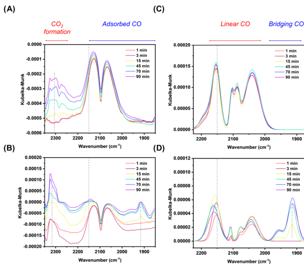
Figure 4. ^{13}\text{CO} DRIFTS data of (A) \text{CeCe}_{70} and (B) \text{CuCe}_{70} in the selected region collected at 200\text{ }^{\circ}\text{C} . Time in legend corresponds to the duration of DRIFTS cell exposure to ^{13}\text{CO}/^{18}\text{O}_2 . Residual DRIFTS data shown in (C) of \text{CeCe}_{70} and (D) of \text{CuCe}_{70} . Gray dotted lines were added to aid the visualization of 2150\text{ cm}^{-1} , while gray dotted arrows demonstrate the evolution of bridging CO peaks at the evolution of \text{CO}_2 .
