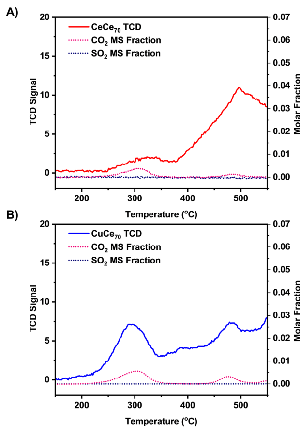
Figure 3. TPR-MS profiles of (A) \text{Ce Ce}_{70} and (B) \text{Cu Ce}_{70} under CO within 150–550 °C range. Remaining molar fraction corresponds to He, the carrier gas for the experiments.
