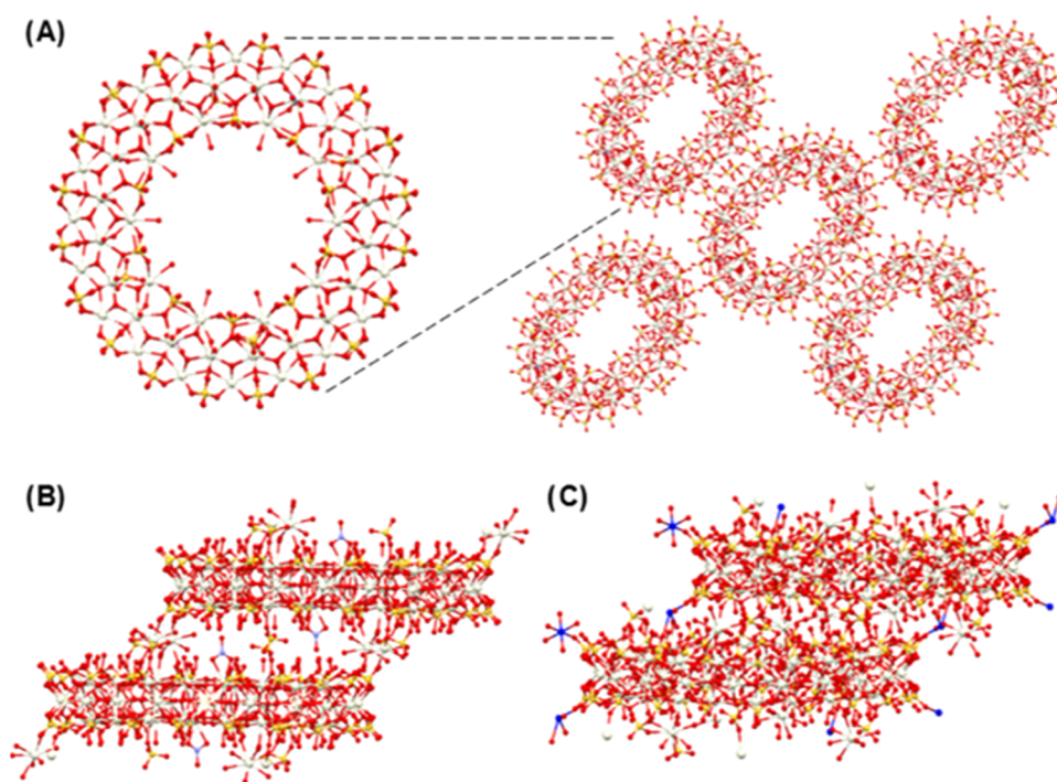
Figure 1. (A) CeCe 70 assembly with the enlarged repeated unit. (B) Interfacial linkage sites between two connected CeCe 70 rings. (C) Linkage sites between two connected CuCe 70 sites. Color scheme: light yellow, Ce; red, O; golden yellow, S; light blue, N; and royal blue, Cu. H atoms are omitted for clarity.
