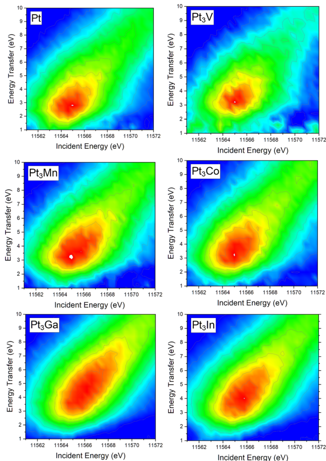
Fig. 1 RIXS plots of Pt and Pt alloy catalysts after reduction at 550 °C in 3.5% H 2 .
