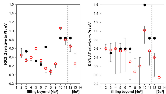
Fig. 4 Direct comparison of simulated RIXS spectra from DFT calculated Pt d-DOS (red) and experimental RIXS spectra (black). Error bars correspond to 30–100% dispersion with 45% dispersion plotted.
