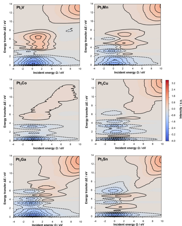
Fig. 3 Simulated difference RIXS plots for a subset of the intermetallics. Each plot is shown at 45% dispersion, relative to a similar 45% dispersion pure Pt particle. The six other intermetallics considered can be found in the ESI† Section S.3.6.
