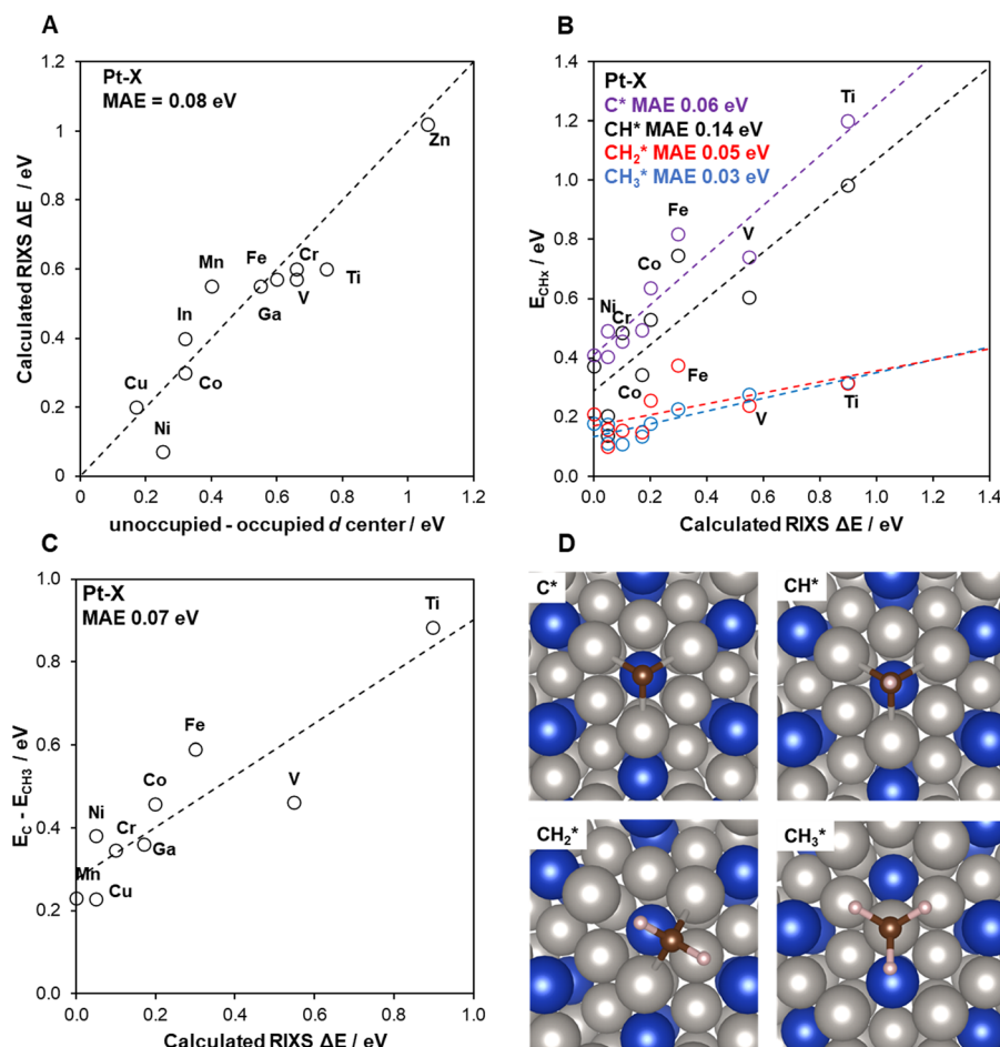
Fig. 5 (A) Correlation between simulated RIXS energy transfer and d separation descriptor across all 2 nm bimetallic particles relative to pure Pt. (B) (C, CH, CH 2 , CH 3 ) energies, and calculated RIXS \Delta E , for the range of Pt–X bimetallics relative to pure Pt. The analysis corresponds to pure surface RIXS (100% dispersion). (C) Relative binding energy of C* and CH 3 *, referenced to pure Pt, for the range of Pt–X bimetallics. (D) Representative adsorption sites on a (111) surface. A complete set of images can be found in Sections S.3.8 and S.3.9 (ESI†). Note that PtZn(011) is not included in these correlations, as it has a different composition and surface termination.
