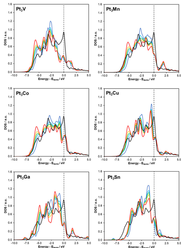
Fig. 2 Projected density of state (DOS) of Pt bulk and surface atoms in intermetallic alloys. The DOS are plotted for increasing dispersion from 0% (red), 30% (yellow), 45% (green), 60% (cyan), and 100% (blue). Pure Pt is shown in black. The six other intermetallics considered can be found in the ESI† Section S.3.4.
