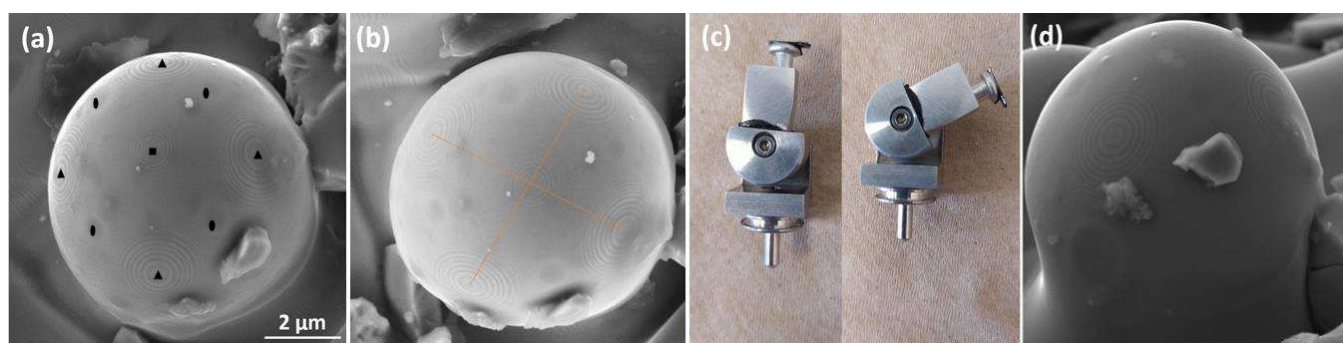
Figure 1 (a) and (b) are SEM images of a spherical particle at random and edge-on orientations. (c) shows the un-tilted (left) and tilted (right) images of the assembled special specimen holder. By using this holder, the sphere can be tilted 70^\circ from the edge-on orientation and the corresponding SEM image is shown in (d).
