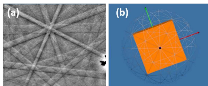
Figure 2 EBSD pattern (a) and the three-dimensional view of the cubic unit cell relative to specimen.
