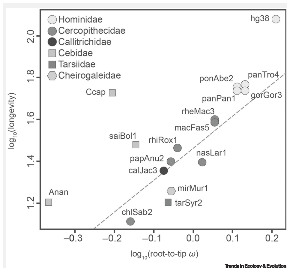
Figure II. Relationship between Rates of Molecular Evolution at the STK17B Locus and Longevity. The broken line represents the best fit from the phylogenetic generalized least squares analysis. Each point corresponds to a single species; symbols are grouped by higher taxon (e.g., filled black circles for Callitrichidae). Adapted from [69].
