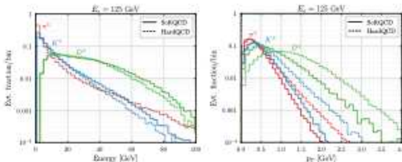
Figure 9. Energy (left) and p_T (right) distributions of mesons produced at an ILC beam dump experiment with an electron beam with energy E_e = 125 GeV hitting a proton at rest. Events are generated with Pythia using the SoftQCD event class (solid curves) and the HardQCD event class (dashed curves). The distributions are normalized such that the total bin count sums to 1.
