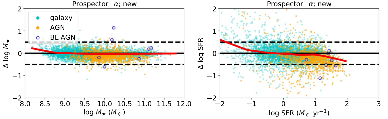
Figure 27. Comparisons between our corrected M_* and SFR (Equations (23) and (24)) and the Prospector- \alpha values. Galaxies generally follow one-to-one relations well while there are still systematic offsets for AGNs, possibly because the Prospector- \alpha fitting attributes some AGN emission to the galaxy component.
