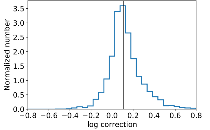
Figure 1. The distribution of the correction factor, defined as the ratio between L_X and the observed X-ray luminosities, for X-ray-detected sources. The vertical black line marks the median correction (0.1 dex).
