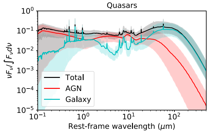
Figure 23. The typical decomposed SED of quasars, constructed from 424 BL quasars in W-CDF-S. This SED is plotted in the same way as for Figure 10, where the cyan and red solid lines represent the galaxy and AGN components, respectively.
