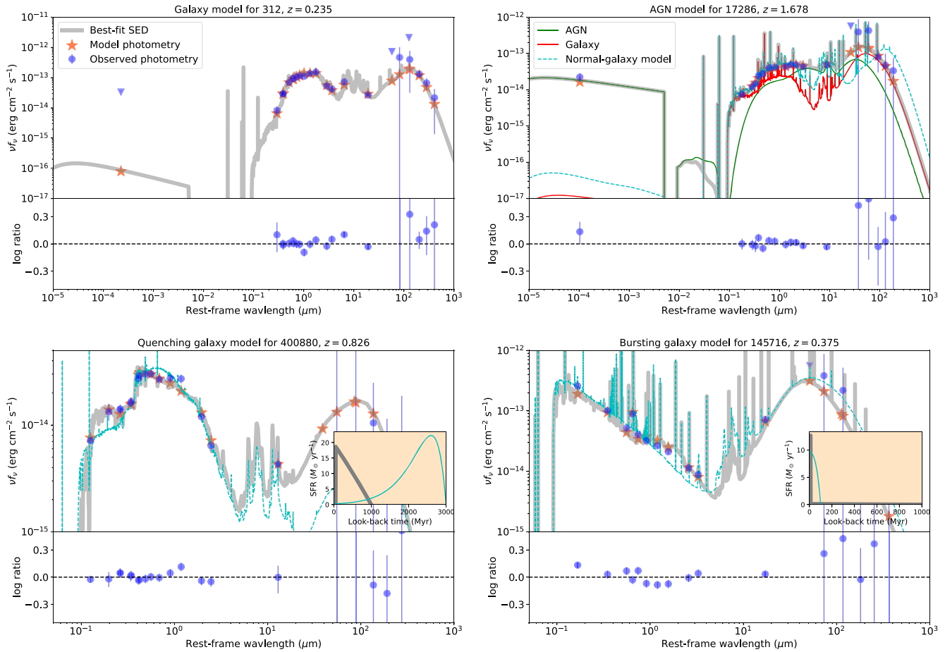
Figure 18. Example rest-frame SEDs fitted by normal-galaxy (top left), AGN (top right), quenching-galaxy (bottom left), and bursting-galaxy (bottom right) templates. The blue points and downward triangles are the observed photometry and upper limits, respectively. The orange stars are the best-fit modeled photometry in the given bands, and the thick gray lines are the best-fit models. The bottom subpanel of each panel shows the logarithm of the ratios of the observed fluxes over the model fluxes. The best-fit model for the AGN example in the top right panel is decomposed into an AGN component (green) and a galaxy component (red). In the panels other than the top left one, we also show the best-fit models with normal-galaxy templates as cyan dashed lines, and they cannot provide acceptable fits to the data. The abscissa axes of the bottom panels are truncated in the UV to help focus on the difference between the BQ and normal-galaxy models, for which the X-ray data cannot provide useful constraints. The inset plots in the bottom panels compare the best-fit SFHs of the BQ-galaxy model (gray) and normal-galaxy model (cyan). For the quenching galaxy in the bottom-left panel, the normal-galaxy model tends to assign most star formation to an early stage, and thus it cannot explain its blue optical color and red UV color simultaneously. Its quenching SFH indicates that it is generally star forming before the quenching but the SFR has dropped significantly recently. For the bursting galaxy in the bottom-right panel, the normal-galaxy model predicts that all the stars were formed recently and hence cannot explain the excess NIR emission; in contrast, the bursting model retains low-level star formation before the burst (i.e., the part of the gray SFH that visually overlaps with the abscissa axis), which contributes to the NIR emission. Another feature of this bursting galaxy is that it has a strong H \alpha line dominating its fourth photometric data point (counted from left to right), and we found that the normal-galaxy model cannot fully explain the excess. H \alpha represents the star formation activity within \sim 10 Myr, and this excessive H \alpha feature does support a strong recent starburst (e.g., Broussard et al. 2019).
