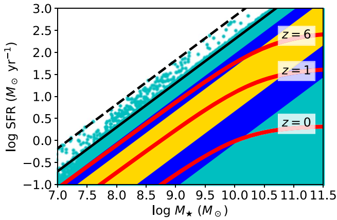
Figure 20. The cyan points are all of our sources in the M_* –SFR plane, which pile up together and visually form linear cuts as the black lines. The black solid and dashed lines correspond to the maximum sSFR allowed ( 10^{-7.70} and 10^{-7.18} \text{ yr}^{-1} ) for our normal-galaxy and BQ-galaxy SFHs, respectively. When only plotting the results from the normal-galaxy fits, all the points will be constrained to lie below the black solid line. The yellow and blue bands represent the 16th–84th and 2.5th–97.5th percentile ranges of sSFR for our star-forming galaxies, respectively. The red curves are the MS at z = 0, 1 , and 6 . All the bands and MS curves are far below the sSFR limits, and thus the apparent sSFR cut does not cause problems.
