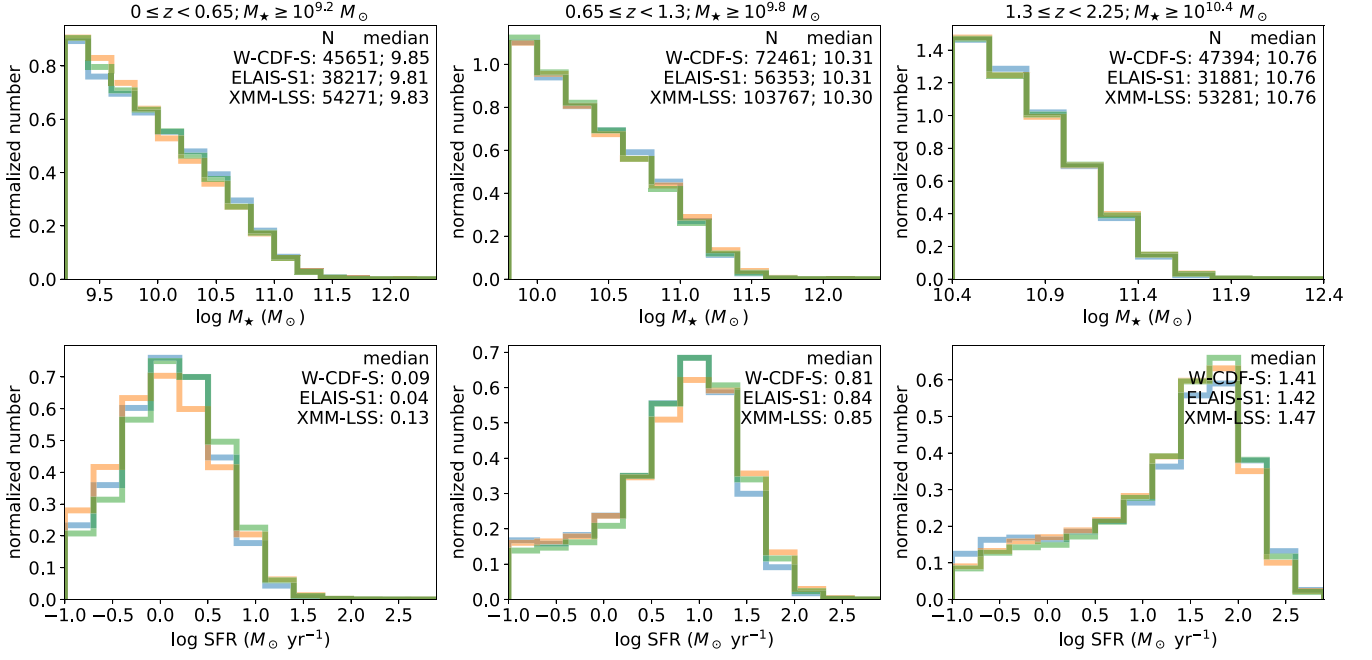
Figure F1. Comparisons of M_* and SFR distributions among our three fields. Sources are separated into three redshift bins with cuts listed in the panel titles. The upper right corner of each panel lists the median value of each distribution, and the numbers of sources plotted are shown in the same locations of the upper panels. The distributions are generally consistent among different fields.
