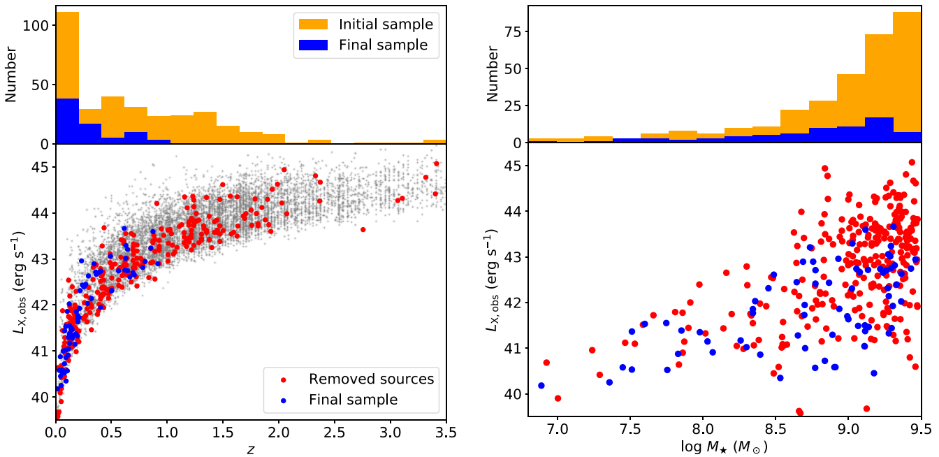
Figure 6. Left: the z – L_{X, \text{obs}} plane. The gray small points are all the XMM-SERVS sources. The blue points are our final active dwarf-galaxy sample, and the red ones are those removed from the initial sample. The top histograms show the redshift distributions of the initial (orange) and final (blue) samples. Right: similar to the left panel but for the M_* – L_{X, \text{obs}} plane, and its top histograms are for the M_* distributions. Our final sample size is much smaller than the initial sample size, highlighting the overall challenges of reliably selecting distant active dwarf galaxies. Selection biases inevitably exist, especially at high redshifts.
