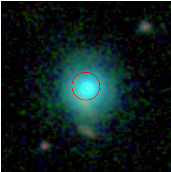
Figure 7. The three-color Hubble image of WCD2044 generated from F814W (blue), F125W (green), and F160W (red) images. The red circle is centered at the XMM-Newton centroid with a radius of 0''.5 .
