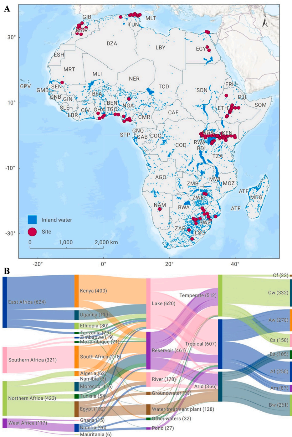
Fig. 1. Geographic distribution of the records of microcystin (MCs) concentration in African waters (A) and Structure (B). Af, tropical rainforest climate; Am, tropical monsoon climate; Aw, tropical savanna climate; Bs, steppe climate; Bw, desert climate; Cf, warm temperate climate with fully humid; Cs, warm temperate climate with dry summer; Cw, warm temperate climate with dry winter.
