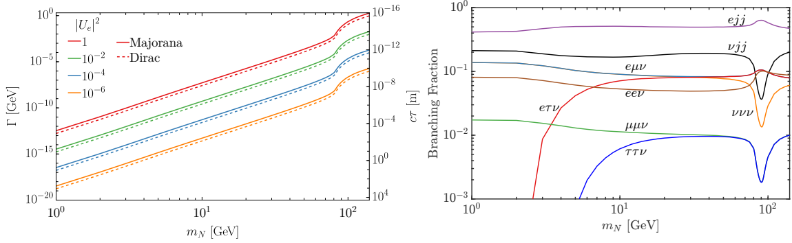
Figure 3. The HNL total decay width (left) and the branching fractions to final states as labeled (right).
