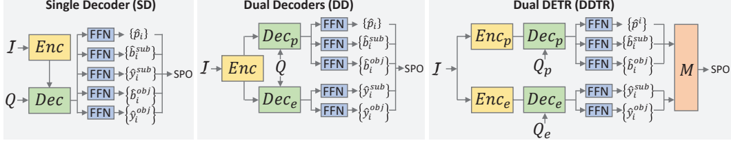
Figure 1: Baselines. Enc , Dec , and M denote the encoder, decoder, and Hungarian matching respectively. (\cdot)_p represents that the instance is for predicate detection, and (\cdot)_e is for entity detection. SPO denotes triplets of \langle \text{subject}, \text{predicate}, \text{object} \rangle .
