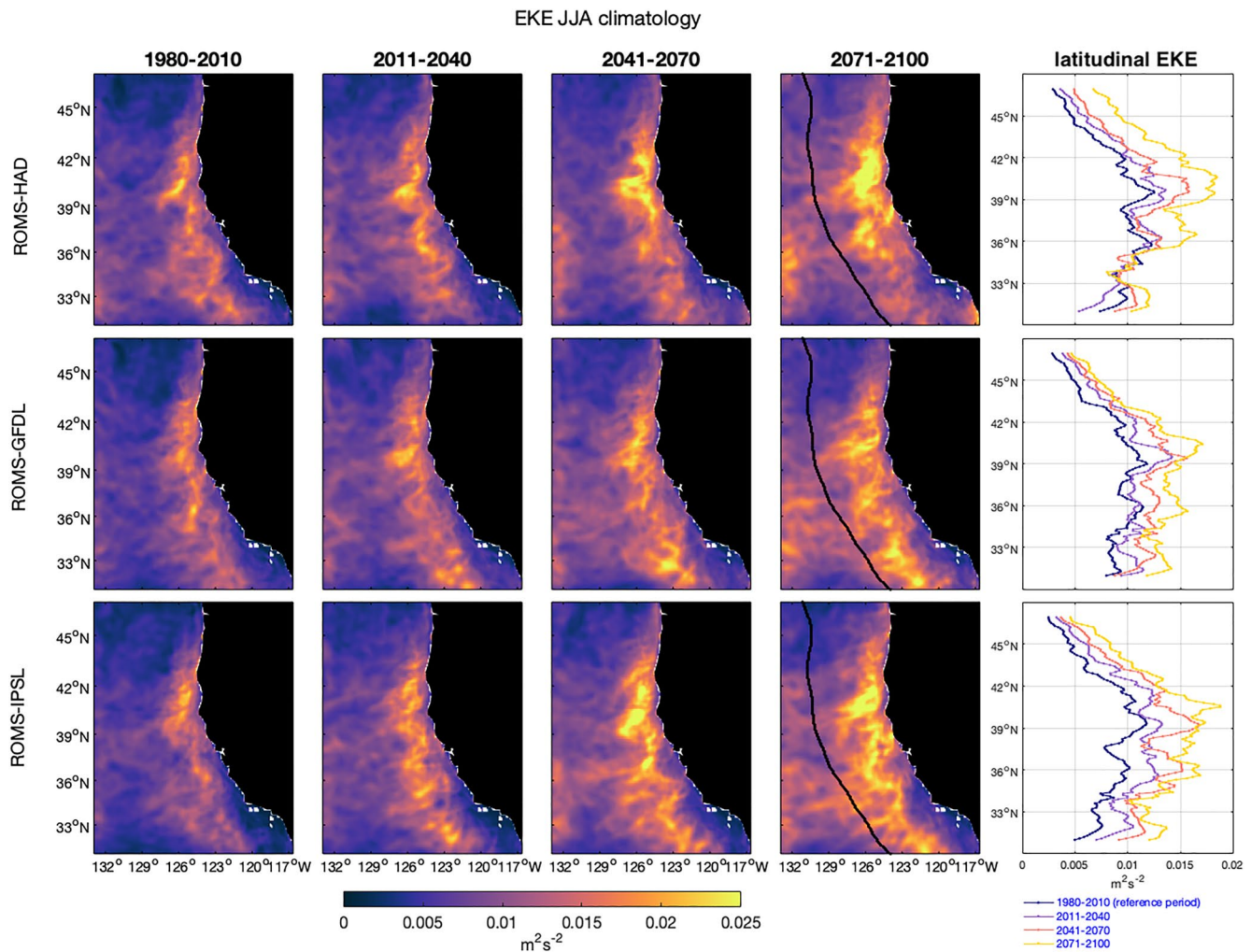
Figure 1. Summer (June, July, and August (JJA)) mean eddy kinetic energy (EKE) for the historical period (1980–2010) and three projected periods (2011–2040, 2041–2070, and 2071–2100) for the three downscaled simulations: (top to bottom) regional ocean model system (ROMS)-HAD, ROMS-GFDL, and ROMS-IPSL. Zonal means of EKE from the coast to 500 km offshore (shown by a black contour in the 2071–2100 maps) are shown in the last column.
