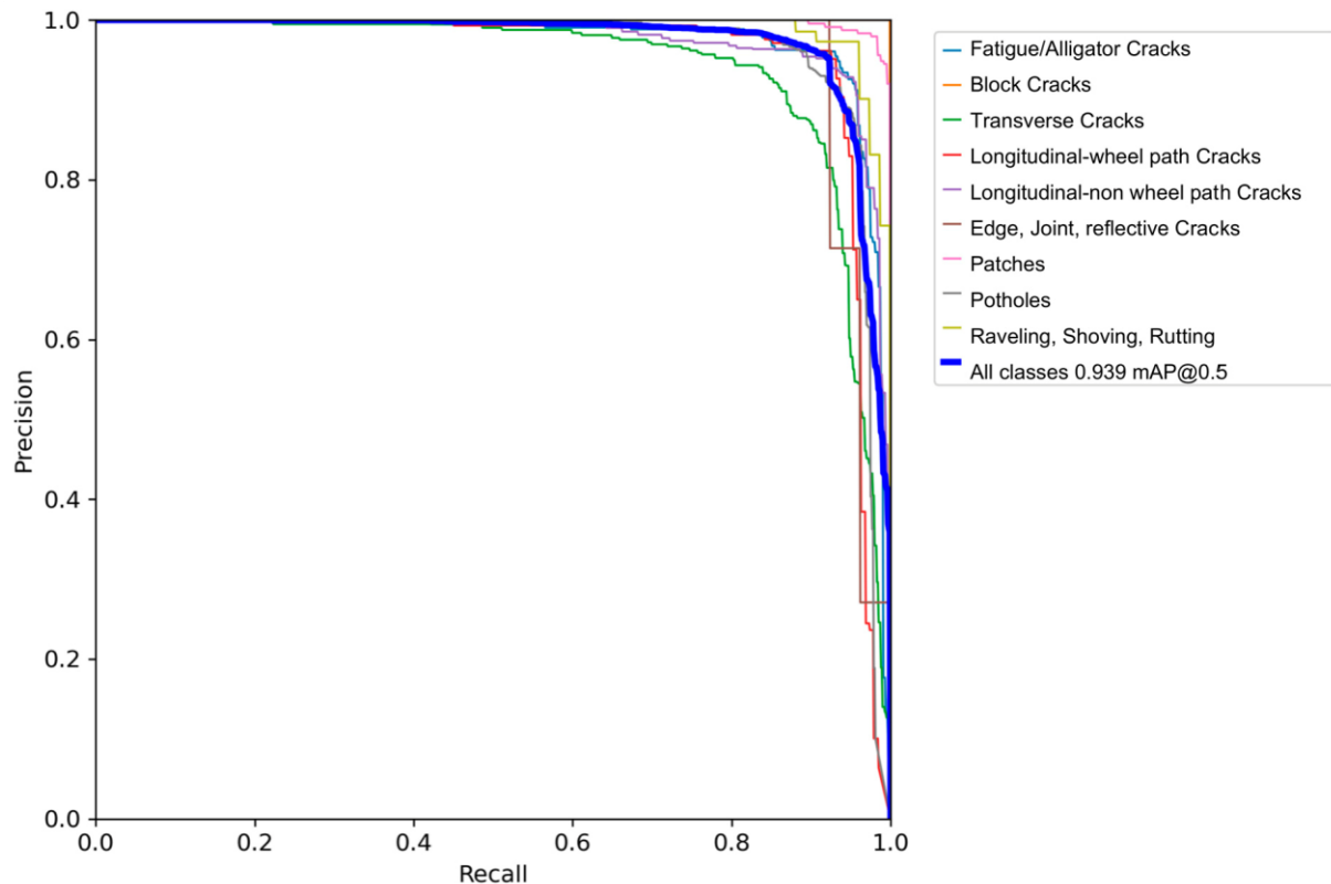
Figure 10. Precision–recall curve.
