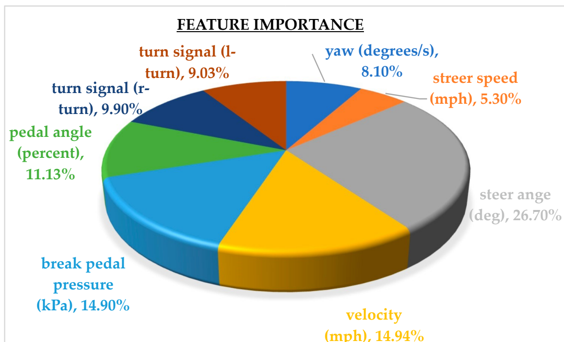
Figure 9. Feature importance to the model predictions.
