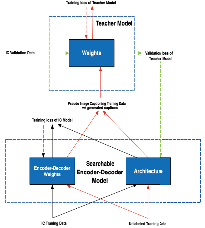
Figure 2: Overview of our Image Understanding by Captioning (IUC) optimization framework. Black, red, and green arrows represent stage 1, stage 2, and stage 3 in our framework, respectively.
