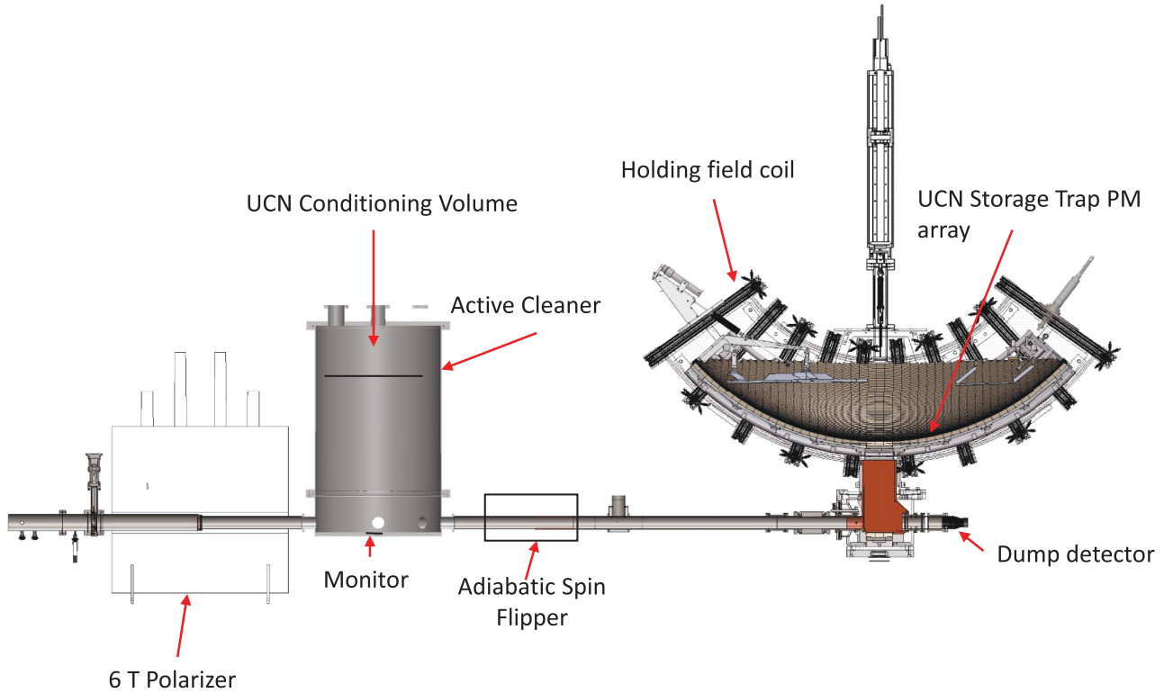
FIG. 1. Experimental layout showing the location of the UCN detectors used in this experiment. The source is off the picture to the left. The dump detector is the primary counter for this experiment.
