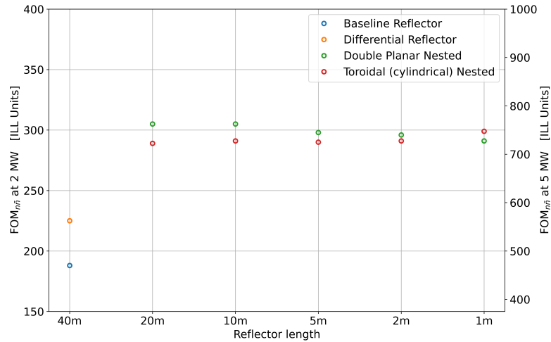
Figure 16. Collected \text{FOM}_{n\bar{n}} s for different reflector geometries. (Left axis) Target power of 2 MW. (Right axis) Target power of 5 MW.
