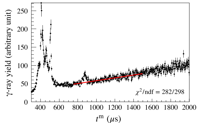
FIG. 9. Histogram of the \gamma -ray yield gated with the full absorption peak of 7132 keV \gamma rays for the single germanium crystal. The solid line shows the fit result of the s -wave and background components.
