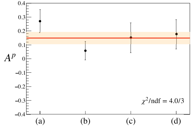
FIG. 12. The values of the angular dependence A^p for each condition. The solid line and colored region show the average value and 1\sigma region, respectively.
