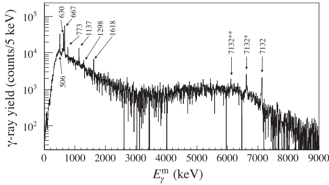
FIG. 5. \gamma -ray spectrum gated with the 3.2 eV p -wave component. The \gamma -ray energies of each peak are also shown. Single and double asterisks indicate single- and double-escape peaks, respectively. The origin of the \gamma -ray peak at 1618 keV was not identified in this study. The detection threshold was around 500 keV.
