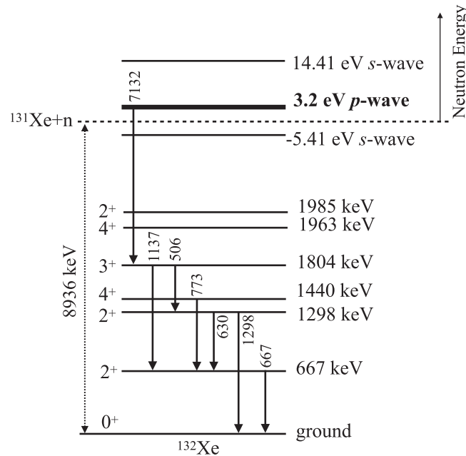
FIG. 6. Decay scheme from the 3.2 eV p -wave resonance of ^{131}\text{Xe} + n to ^{132}\text{Xe} . The dashed line shows separation energy of ^{131}\text{Xe} + n . The excited states less than 2000 keV are depicted.
