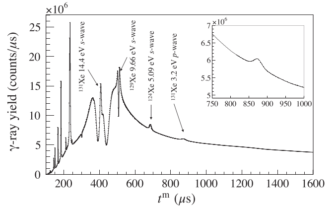
FIG. 3. \gamma -ray counts as a function of t^m with the ^{131}\text{Xe} target. In the inset, an enlarged view of the 3.2 eV p -wave resonance is shown. The peak at 410 \mu\text{s} is considered to originate from neutrons passing through the gap between the collimator and the ^{131}\text{Xe} filter.
