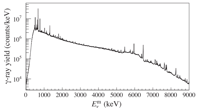
FIG. 4. \gamma -ray spectrum.
