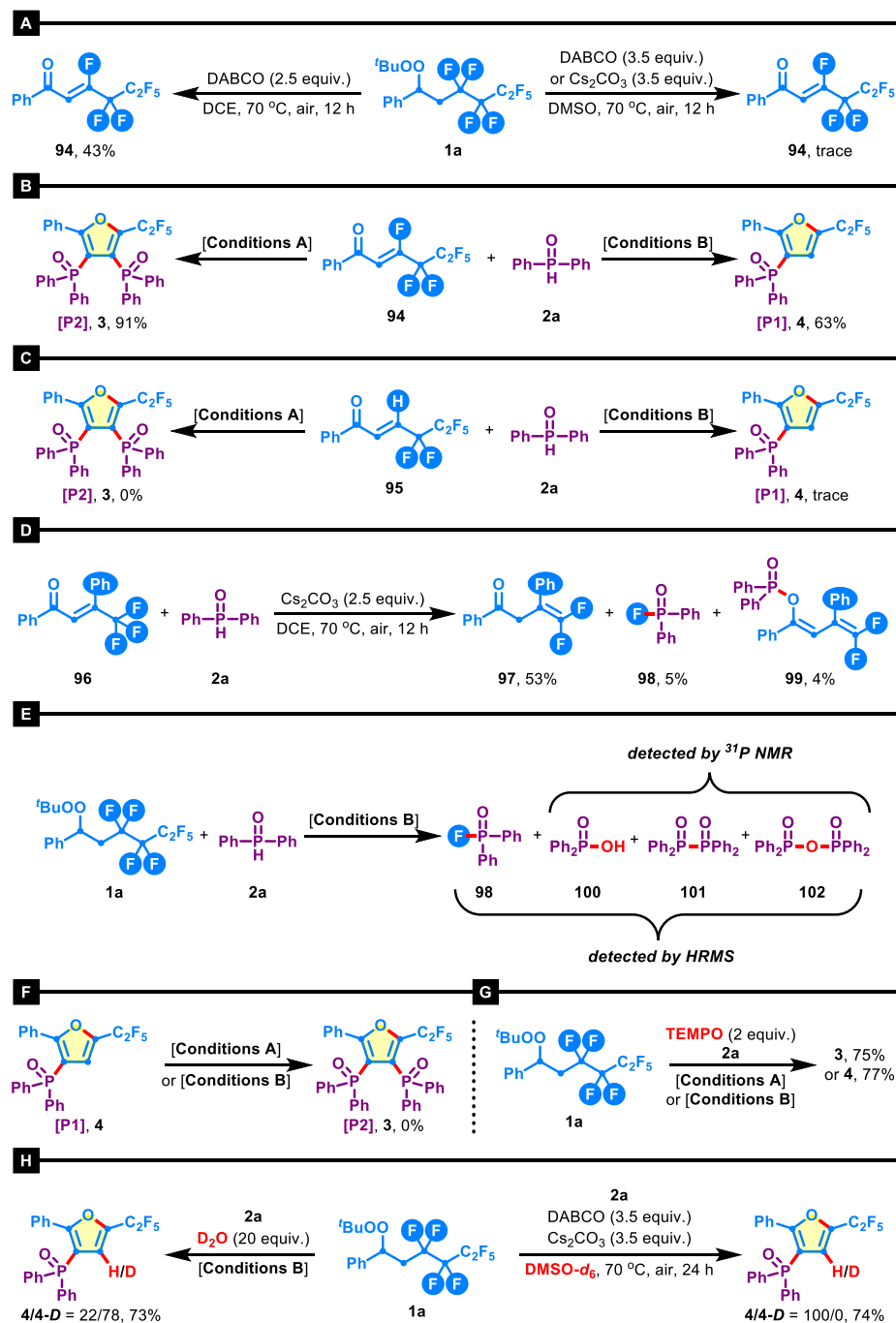
Figure 4. Mechanistic studies. A The formation of unsaturated ketone intermediate. B The defluorinative transformation of unsaturated ketones to furan products. C The necessity of vinyl fluoride for these transformations. D The role of \text{HP}(\text{O})\text{Ph}_2 as a defluorinative reagent. E HRMS and ^{31}\text{P} NMR analysis of the reaction mixture. F Direct phosphorylation of monophosphorylated product was unsuccessful. G TEMPO-trapping experiment. H Deuterium-labeling experiments.
