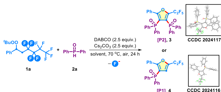
Figure 2. Defluorophosphorylation protocols. A Michaelis-Arbuzov-type phosphonate synthesis starting from alkyl fluorides. B Phosphorylation of non-activated aryl fluorides via concerted S N Ar pathway or radical pathway. C Phosphorylation of CF 3 -substituted alkenes via an S N 2' pathway. D Defluorophosphorylation of perfluoroalkyl ketones. E Successive defluorination and dual sulfonylation relay of fluoroalkyl peroxides. F Classic Atherton-Todd reaction through phosphoryl-anion-initiated dehalogenation. G New design for the synthesis of C3,4-diphosphorylated and C4-phosphorylated furan derivatives through selective defluorophosphorylation. H Key results in reaction optimization. a Reaction conditions: (1-( tert -butylperoxy)-3,3,4,4,5,5,6,6,6-nonafluorohexyl)benzene ( 1a , 0.36 mmol), diphenylphosphine oxide ( 2a , 0.3 mmol), DABCO (0.75 mmol), and Cs 2 CO 3 (0.75 mmol) in solvent (2.0 mL) at 70 °C for 24 h under air. b Yields were determined by NMR analysis with 1,4-dimethoxybenzene as an internal standard. c Isolated yield. d 1a (0.3 mmol), 2a (0.9 mmol), DABCO (1.05 mmol), and Cs 2 CO 3 (1.05 mmol) were used.
