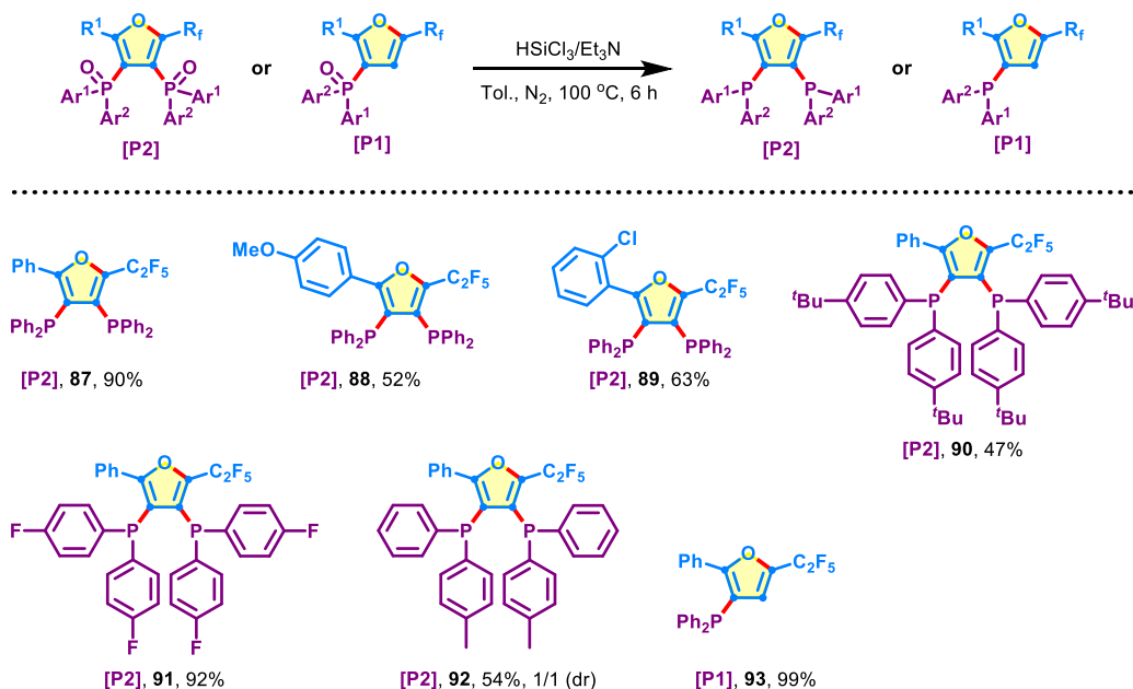
Figure 3. Scale-up synthesis and further transformations. A Scale-up synthesis of phosphoryl furans 3 and 4 . B Synthesis of complex products. C Further reductive transformation of phosphoryl furans to trivalent phosphines.
