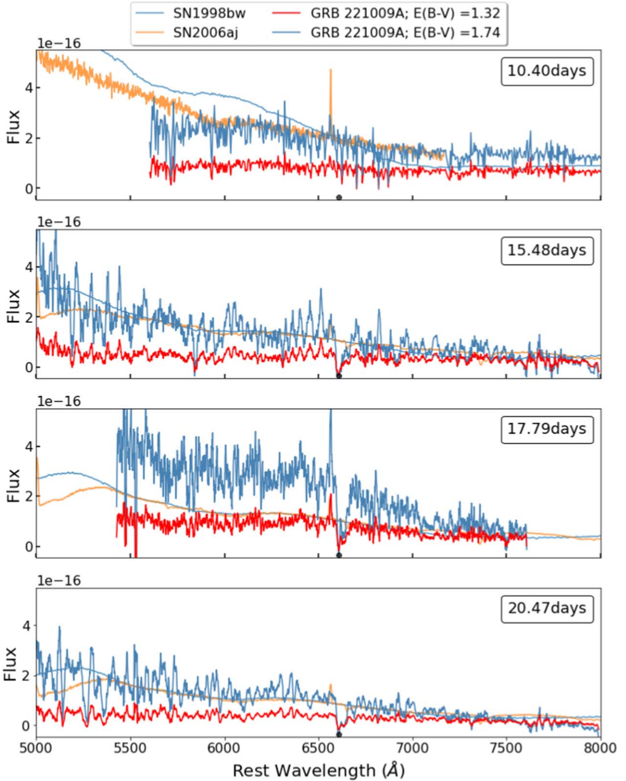
Figure 8. Smoothed spectra of GRB 221009A compared to two SNe, SN 1998bw and SN 2006aj, which were both associated with GRBs. The spectra have been corrected for extinction using the two values used throughout this work ( E(B - V) = 1.32 mag and E(B - V) = 1.74 mag) and have been corrected for their redshift appropriately. All the spectra are calibrated to the photometry of GRB 221009A at the same phase, and the GRB afterglow contribution is subtracted. The four panels are for four different times since the GRB trigger time: 10.40 days, 15.48 days, 17.49 days, and 20.47 days. The spectrum of GRB 221009A at 10.40 days is from HET, and the spectra at 15.48 days, 17.49 days, and 20.47 days are from the MMT. Although the initial HET spectrum bears some resemblance to SN 1998bw in the high-extinction scenario, overall there are no clear SN features present.
