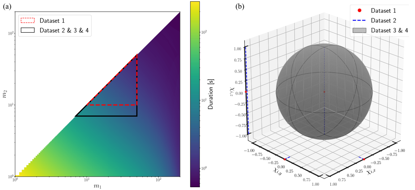
FIG. 1. An illustration of the range for the intrinsic parameters covered by this challenge. The left panel (a) shows a typical range for the component masses used by state-of-the-art searches [14]. The color indicates the duration of the waveform from 20 Hz. The triangles show the parameter regions covered by this challenge. The right panel (b) shows the component-spin \chi_i distribution of the different datasets in this challenge.
