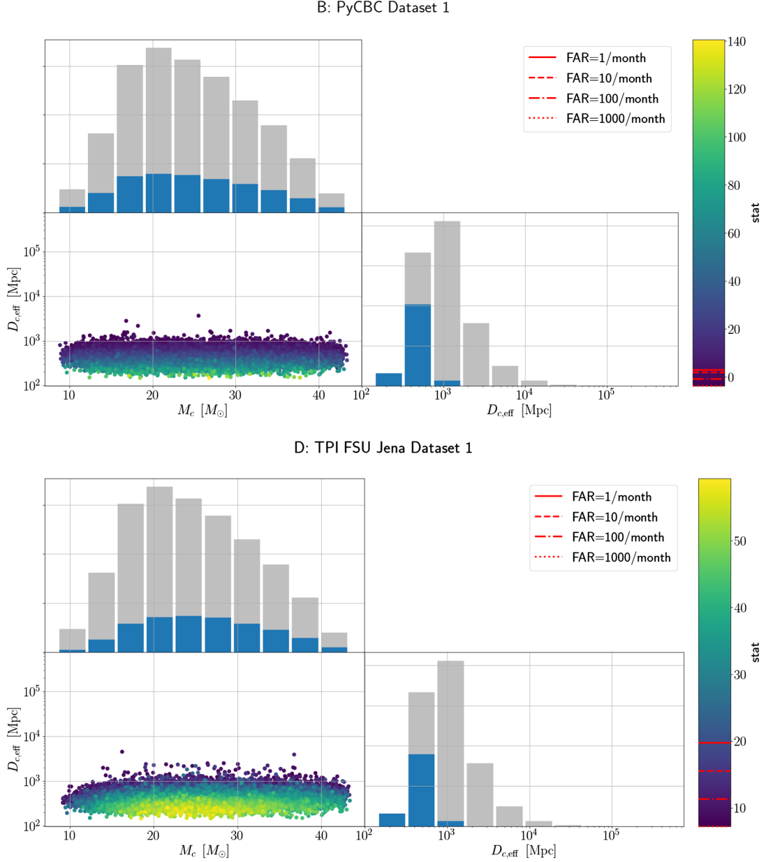
FIG. 4. The injections from dataset 1 identified by the PyCBC and TPI FSU Jena submissions with a FAR \leq 10^3 per month in the chirp-mass M_c versus decisive effective chirp-distance D_{c,\text{eff}} plane. The blue bars in the histograms show the one-dimensional marginal distributions of the found injections. The gray bars show the distribution of injected signals, including those missed by the search. The color shows the “stat” value attributed to the injection by the algorithm. The red lines in the color bar highlight the thresholds on the “stat” to achieve different FARs.
