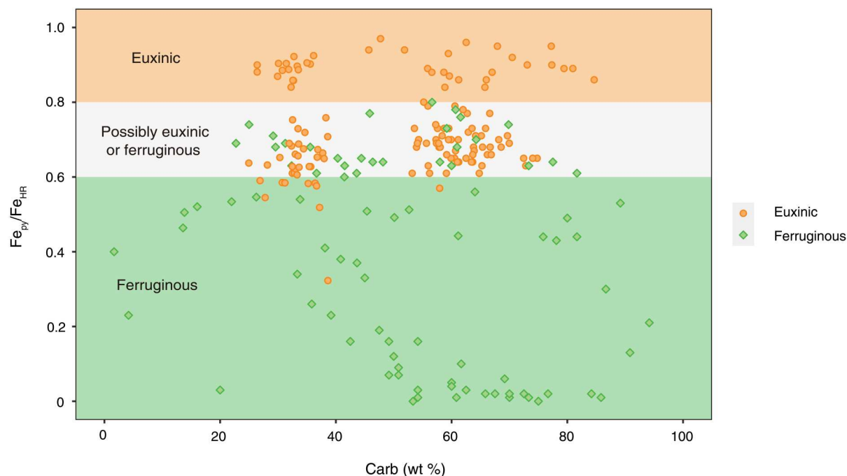
Fig. 4. \text{Fe}_{\text{py}}/\text{Fe}_{\text{HR}} ratios plotted against carbonate percentage for independently assessed euxinic and ferruginous samples. Modern and ancient samples with \text{Fe}_T \geq 0.5\% were plotted. The data compilation confirms that the recently proposed euxinic/ferruginous threshold (0.6 to 0.8) is valid for distinguishing euxinic versus ferruginous conditions in carbonate samples. See table S1 for data sources and independent assessment of redox conditions.
