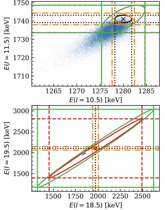
FIG. 9. A 2D cut of the posterior predictive distribution at N^4\text{LO} and k_{\text{max}} = 10 for ^{169}\text{Er} and I_{\text{max}} = 17.5 (top panel) and at k_{\text{max}} = 18 for ^{235}\text{U} and I_{\text{max}} = 23.5 (bottom panel). The blue dots show the energies calculated from the distribution of the LECs. The black cross shows the experimental value and the black lines and black ellipse shows the corresponding experimental uncertainty. The remaining ellipses and lines show the truncation error and the experimental error added in quadrature. (All the ellipses are centered at the experimental value.) The orange, red and green account for 1, 2 and 6 omitted terms in the theory error respectively. (In the top panel the red ellipse is completely covered by the green ellipse.)
