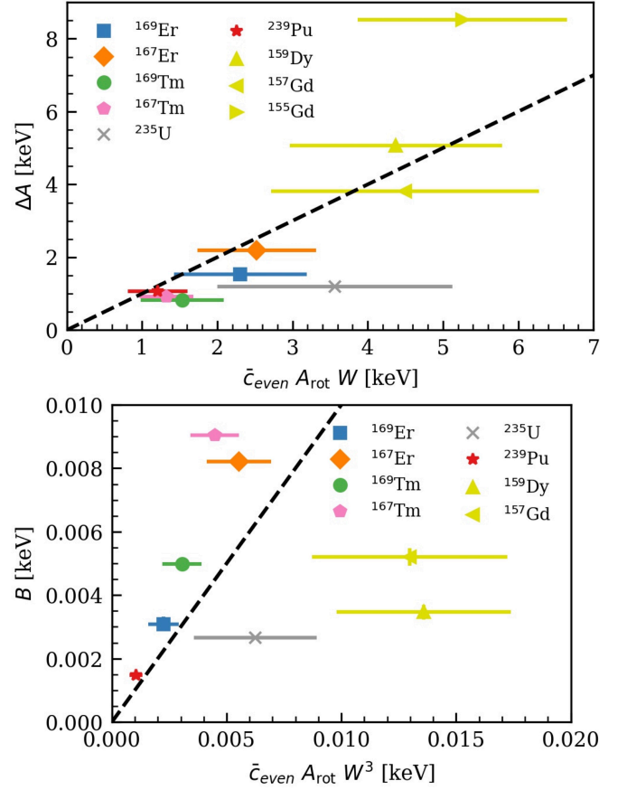
FIG. 11. The size of the \text{N}^2\text{LO} LEC, \Delta A , (top panel) and the \text{N}^4\text{LO} LEC, B , (bottom panel), on the y-axis, compared to its expected size from the EFT power counting, on the x-axis. Error bands on the LEC distribution are small and can not be seen on the plot. The error bands on the x-axis encompass uncertainties between on the 16th and 84th percentiles. Different nuclei are labeled in the legend of the plot. The black dashed line has \text{slope} = 1 and is plotted to facilitate comparison of prior expectation with results from the posterior. The yellow colored symbols are results for rotational bands with bandheads K = 3/2 , all the others are K = 1/2 bands. ^{99}\text{Tc} and ^{183}\text{W} are outliers and we exclude them from the both plots. We also exclude ^{155}\text{Gd} from the bottom plot only. (LECs values for these nuclei can be found in Table I.)
