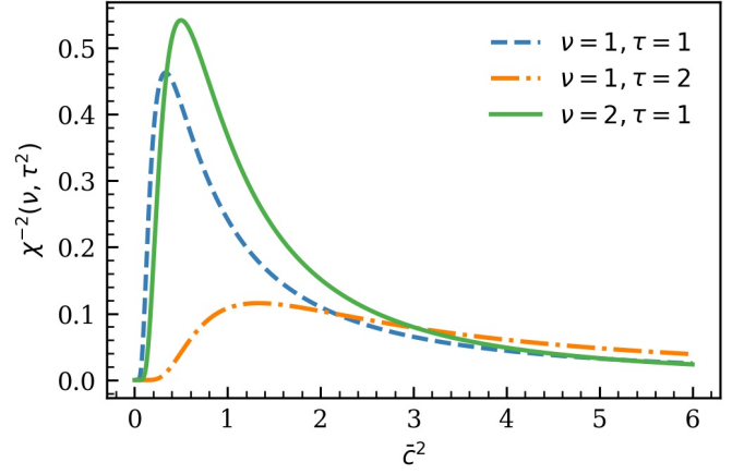
FIG. 2. Prior distribution of the size of the dimensionless natural coefficients, \bar{c} .
