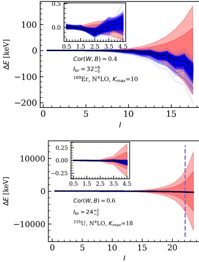
FIG. 8. The posterior predictive distribution for energy-level residuals at N^4\text{LO} and k_{\text{max}} = 10 for ^{169}\text{Er} and I_{\text{max}} = 17.5 (top panel) and at k_{\text{max}} = 18 for ^{235}\text{U} and I_{\text{max}} = 23.5 (bottom panel). The dark and light red bands show the truncation error plus the experimental error at 68% and 95% credible levels respectively. The lighter blue lines connect the energy residuals calculated from the distribution of the LECs. The solid black line represents the median of the distribution and the dashed lines indicate the 16th and 84th percentiles. The correlation shown on the plot is the highest correlation between any LEC and any error-model parameter. I_{\text{br}} was determined from the distribution of W . The dashed purple line shows the lower limit of I_{\text{br}} . The insert on the plot shows the residuals on the first 5 levels with an altered y-axis scale.
