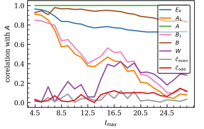
FIG. 6. Correlations between LECs and error-model parameters as a function of I_{max} , resulting from the analysis on the lowest K = 1/2 rotational band in ^{239}\text{Pu} at N^4\text{LO} with k_{max} = 10 .
