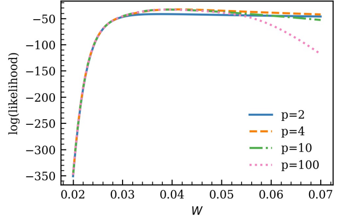
FIG. 1. Comparing the Log of the likelihood when accounting for different number of omitted terms, p , in the theory error. Apart from W , the parameters that enter the likelihood were chosen to be the median parameters after we had sampled the posterior distribution for ^{169}\text{Er} .
