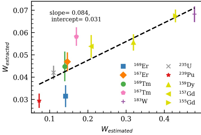
FIG. 12. The extracted inverse breakdown scale W from the marginalized posterior distribution obtained by sampling compared to its naively expected size. The expected size is taken to be the maximum of E_{\text{rot}}/E_{\text{sp}} and E_{\text{rot}}/E_{\text{vib}} . The dashed black line shows the best linear fit and its parameters are printed on the plot. The yellow colored symbols are results for rotational bands with bandheads K = 3/2 , all the others are K = 1/2 bands. ^{99}\text{Tc} is an outlier and we exclude it from the plot (its values could be seen in Table II)
