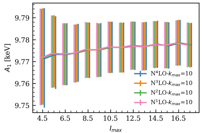
FIG. 4. Posteriors for A_1 describing ^{169}\text{Er} as a function of I_{\text{max}} at different EFT orders. The solid line connects the median values and the error bands encompass the 16th and 84th percentiles of the marginalized distribution.
