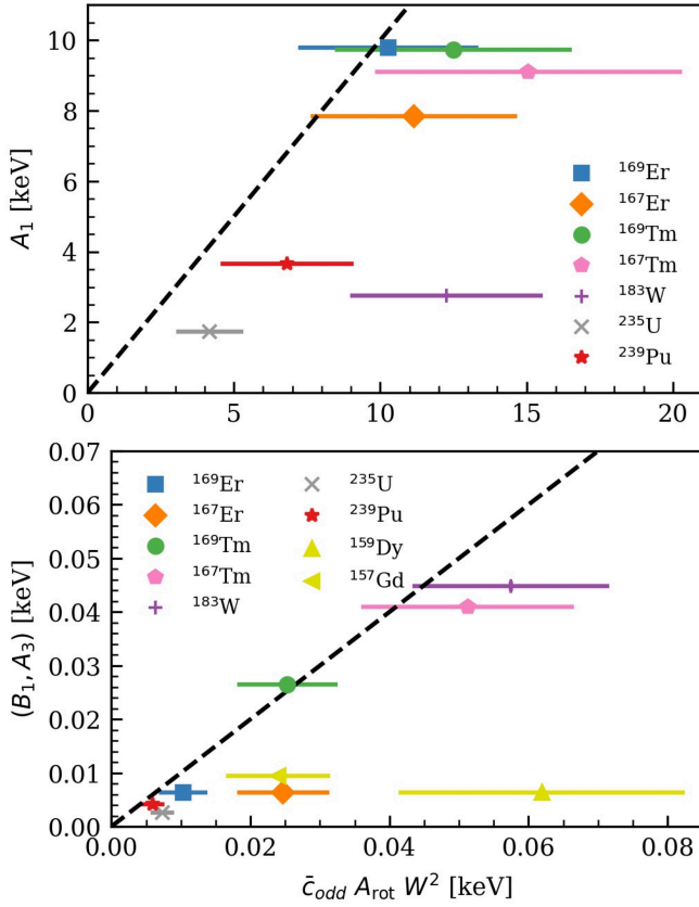
FIG. 10. The size of the NLO LEC, A_1 , (top panel) and the \text{N}^3\text{LO} LEC, B_1 for K = 1/2 bands and A_3 for K = 3/2 bands (bottom panel), on the y-axis, compared to its expected size from the EFT power counting, on the x-axis. Error bands on the LEC distribution are small and can not be seen on the plot. The error bands on the x-axis encompass the 16th and 84th percentiles. Different nuclei are labeled in the legend of the plot. The black dashed line has \text{slope} = 1 and is plotted to facilitate comparison of prior expectation and results from the posterior. The yellow colored symbols are results for rotational bands with bandheads K = 3/2 , all the others are K = 1/2 bands. K = 3/2 rotational bands do not have a parameter A_1 and we do not have them in the top panel. ^{99}\text{Tc} and ^{155}\text{Gd} are outliers and we exclude them from the plots. (LECs values for these nuclei can be found in Table I.)
