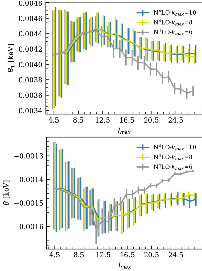
FIG. 5. Posteriors for B_1 and B describing ^{239}\text{Pu} as a function of I_{max} for different values of k_{max} . The solid line connects the median values and the error bands encompass the 16th and 84th percentiles in the marginalized distribution.
