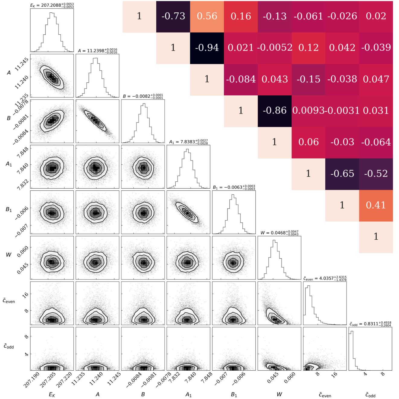
FIG. 3. Corner plot for the marginalized distributions of the LECs and the error-model parameters at N^4\text{LO} for ^{167}\text{Er} including all adopted rotational levels ( I_{\text{max}} = 16.5 ) and accounting for 6 omitted terms in the theory error. The insert in the top right corner show the correlations between posterior parameters. The order of the parameters on the corner plot is the same on the correlations plot. (Here E_K and all the EFT LECs are expressed in keV. The error-model parameters are dimensionless.)
