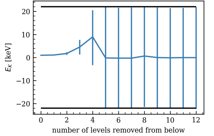
FIG. 7. The distribution of E_K for ^{169}\text{Er} at N^4\text{LO} and k_{max} = 10 as we successively remove the lowest energy levels from the data set D . The solid blue line connects the median values and the error bands encompass uncertainties between on the 16th and 84th percentiles of the samples in the marginalized distribution. The solid black lines show to size of the standard deviation set with the Gaussian prior on E_K .
