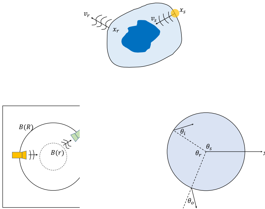
Figure 2. Left: Illustration of the setup for numerical experiments; right: sketch of the definition of the angles on the circle \partial B(R) used to parameterize the data.
