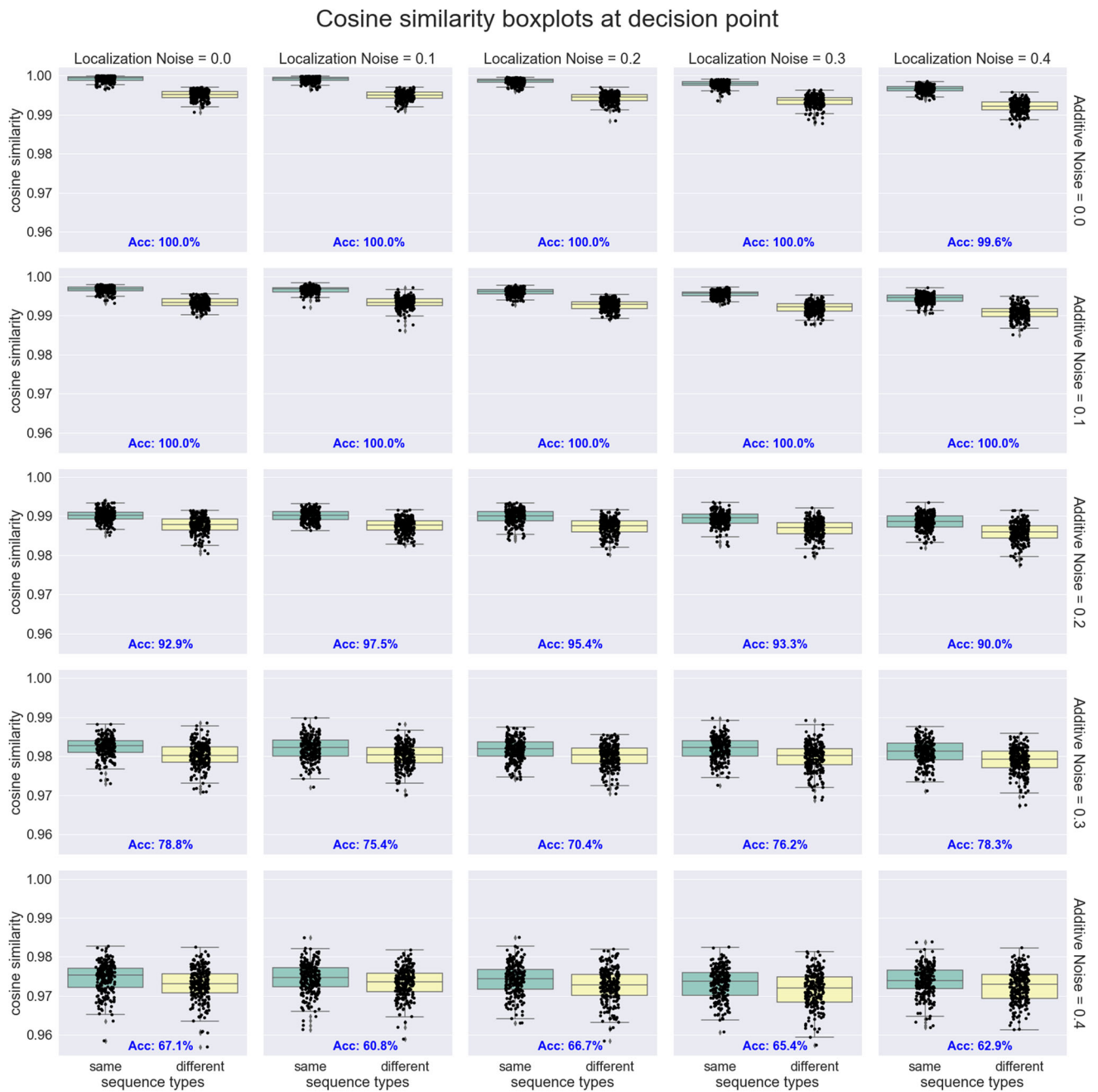
Fig. 13 Experiment 3. Noisy cosine similarities. The figure shows a table of boxplots for different noise levels illustrating the cosine similarities between reservoir states of the same and different sequence types (FSS and SFS) at the decision point. Each boxplot is composed of
