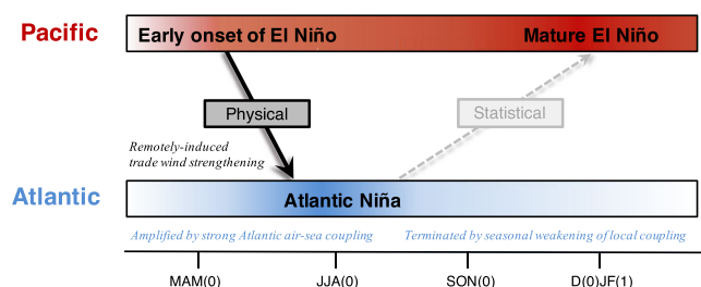
Figure 4. Schematic illustration explaining the inter-basin Pacific El Niño and Atlantic Niño relationship. An early-onset El Niño event during late boreal spring to early summer drives an ensuing summer Atlantic Niña event. Subsequently, the El Niño event shows full manifestation in winter, which is automatically correlated with the previous summer equatorial Atlantic sea surface temperature variability. The same mechanism works for a developing La Niña driving a summer Atlantic Niño.
