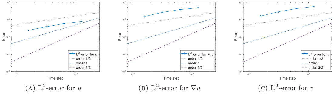
FIG. 3. (Example 6.1) Rates of convergence of the (1, \frac{1}{4}) -scheme with \sigma(v) = \frac{3}{2}v and F \equiv 0 .
