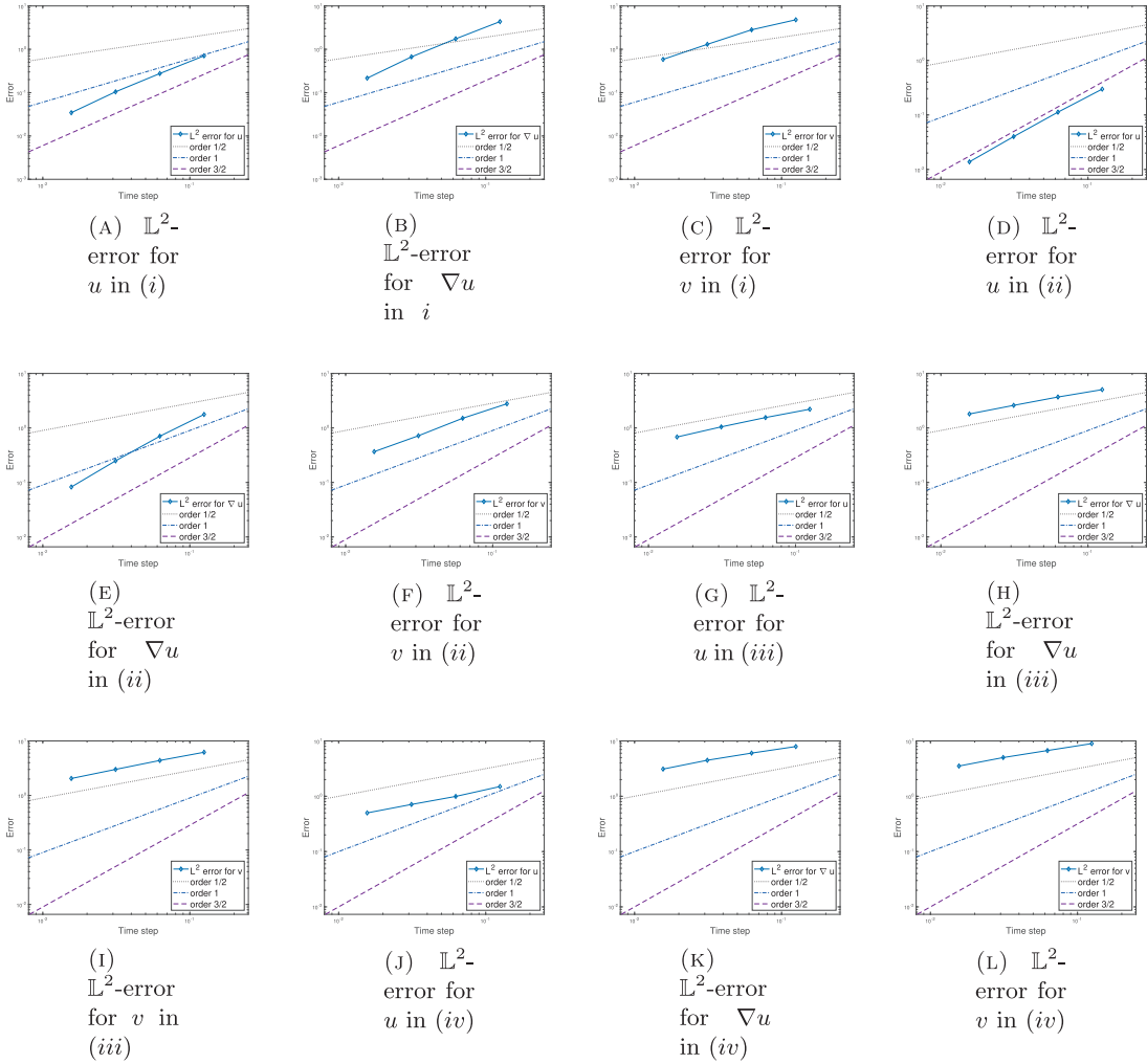
FIG. 4. (Example 6.2) Rates of convergence of the (1, \frac{1}{4}) -scheme.
