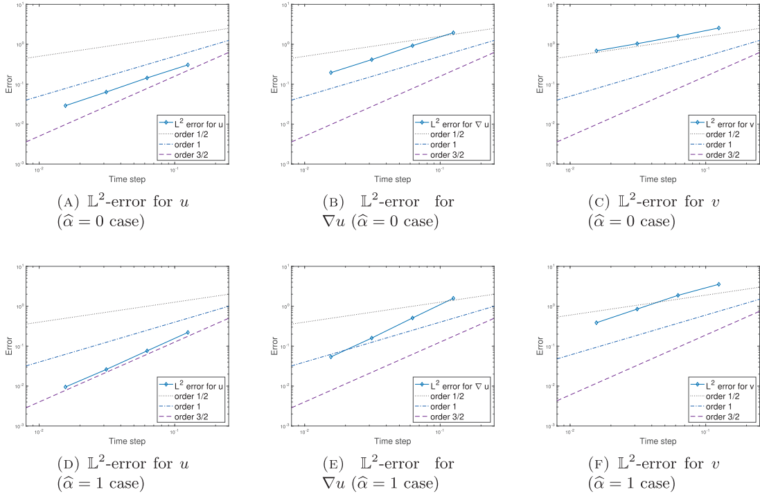
FIG. 2. ( Example 1.2 ) Temporal rates of convergence for the schemes (1.9)–(1.10) with F \equiv 0 and \sigma(u) = 2 \sin(u) ; \hat{\alpha} = 0 in (A), (B), (C) and \hat{\alpha} = 1 in (D), (E), (F); discretization parameters: h = 2^{-7} , k = \{2^{-3}, \dots, 2^{-6}\} , MC = 3000.
