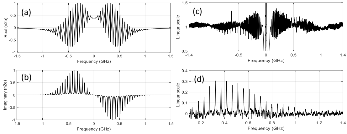
Fig 2. (a) and (b): amplitude normalized real and imaginary parts of n_{2e} . (c) spectrum of recovered complex optical field with 1.5GHz linear chirp. (d) frequency-dependent loss due to electrostriction obtained by subtracting the spectrum shown in (c) from its complex conjugate.
