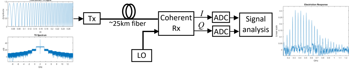
Fig 1. Experimental Setup
