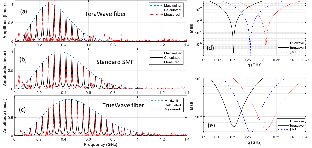
Fig 3. (a – c): measured (dotted lines) and calculated (solid lines) frequency-dependent loss of electrostriction for 3 types of fibers. Dashed lines: Maxwellian fitting. (d) normalized MSE between calculated envelope of electrostriction resonance and Maxwellian distribution with varying q value, (e) normalized MSE between measured envelope of frequency dependent loss and Maxwellian distribution with varying q value
